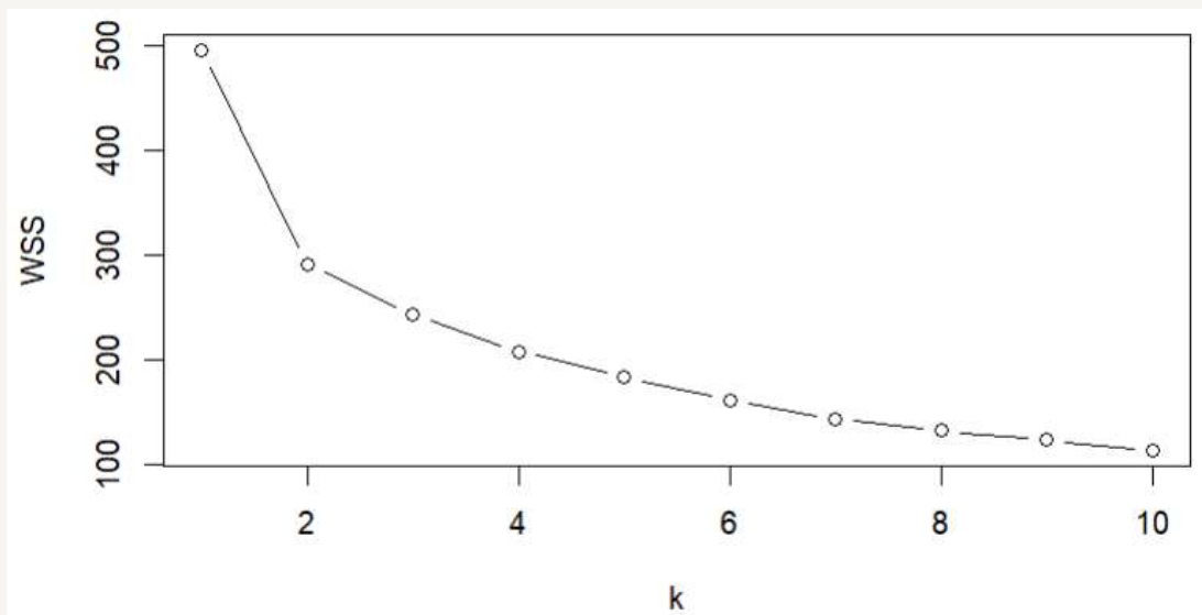
WSS (Within Sum of Squares) — 2023
