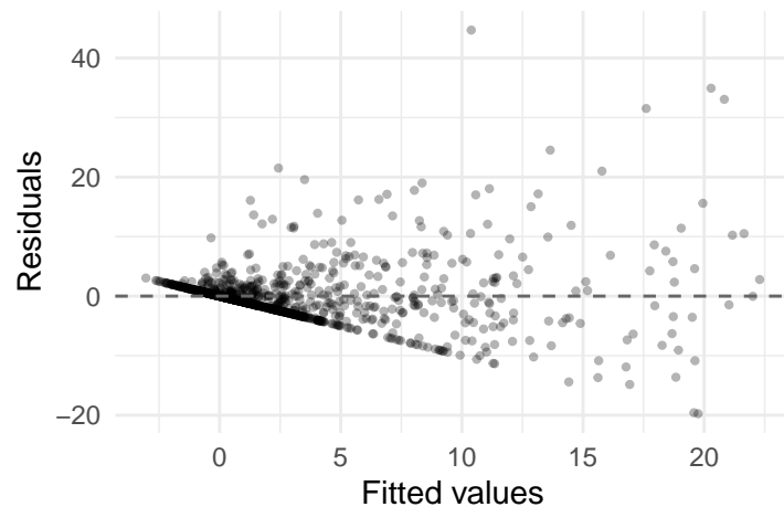
Leish aggregated model (Eq. 2)
