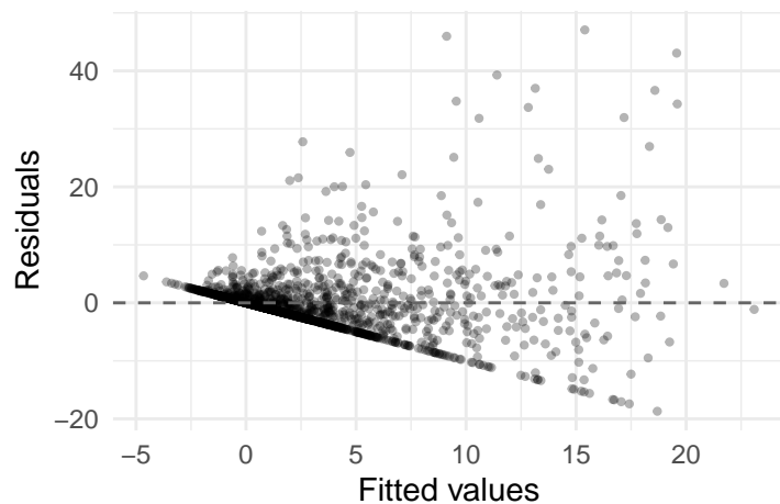
Leish yearly model (Eq. 1)
