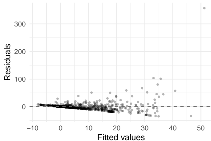
Dengue aggregated model (Eq. 2)
