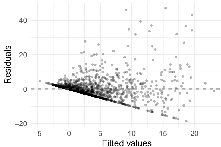
Leish yearly model (Eq. 1)
