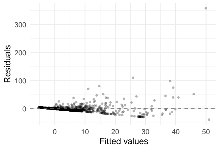
Dengue yearly model (Eq. 1)
