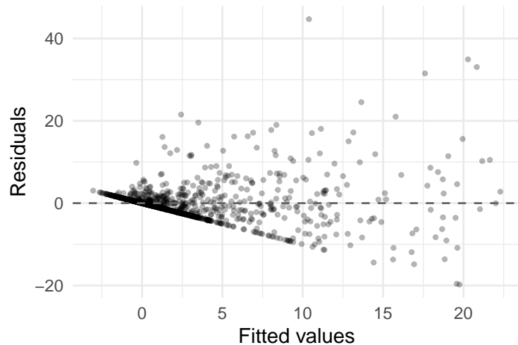
Leish aggregated model (Eq. 2)
