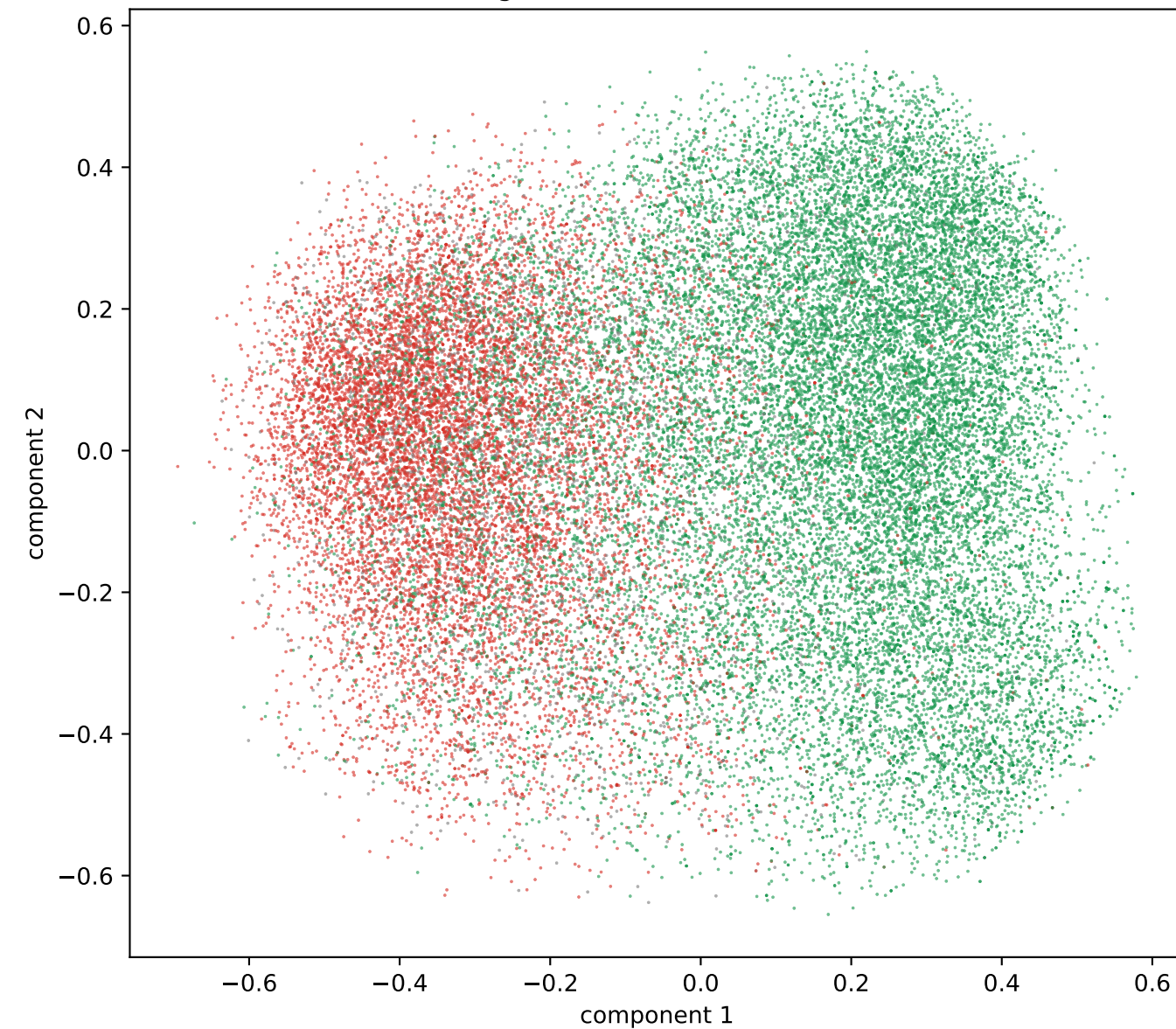
Multilingual MiniLM - PCA (sentiment)
