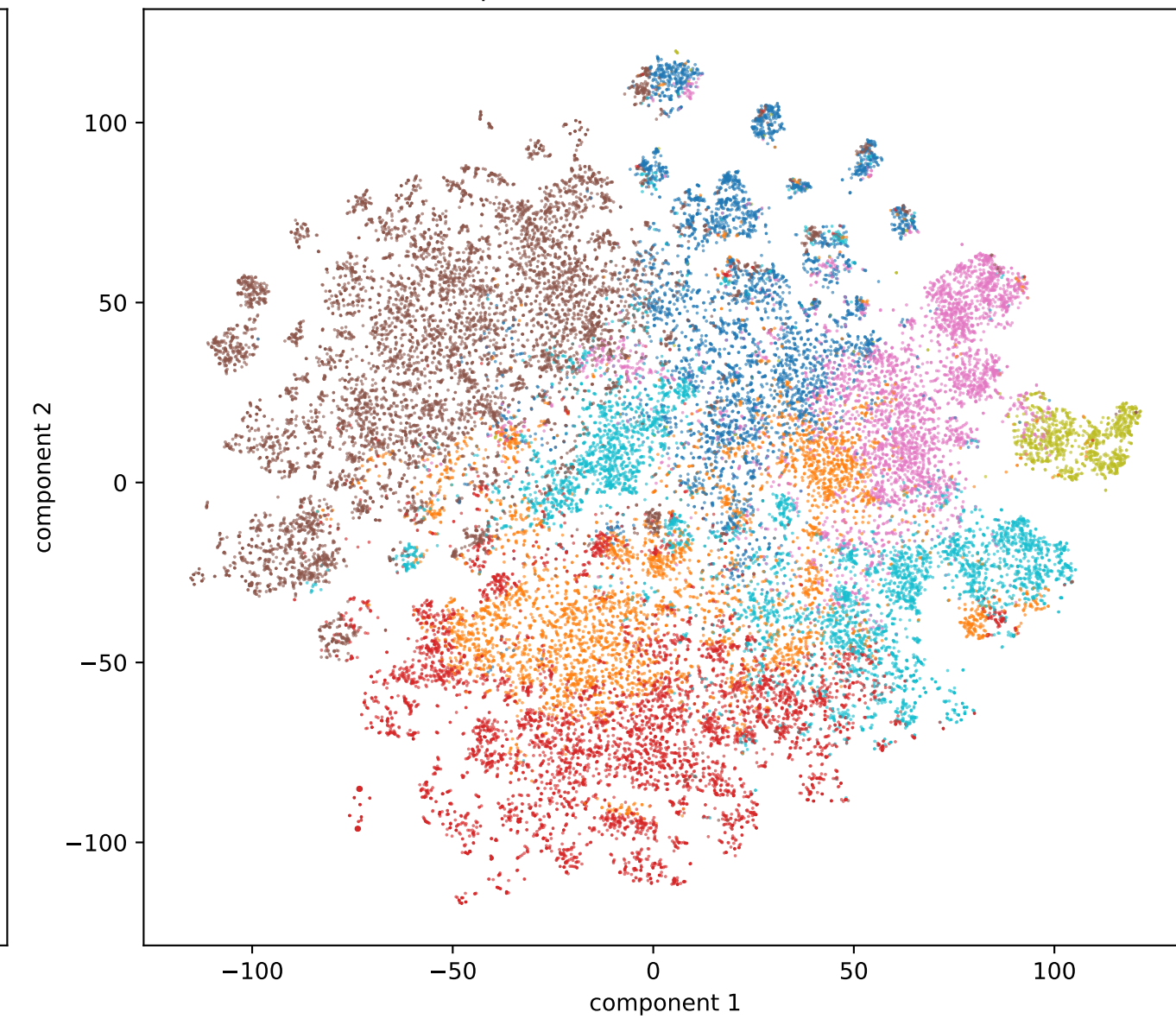
OpenCLIP text - tSNE (cluster)
