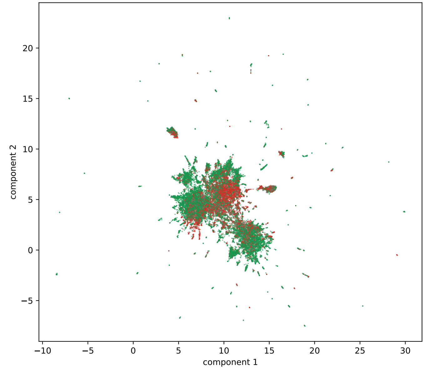
OpenCLIP text - UMAP (sentiment)
