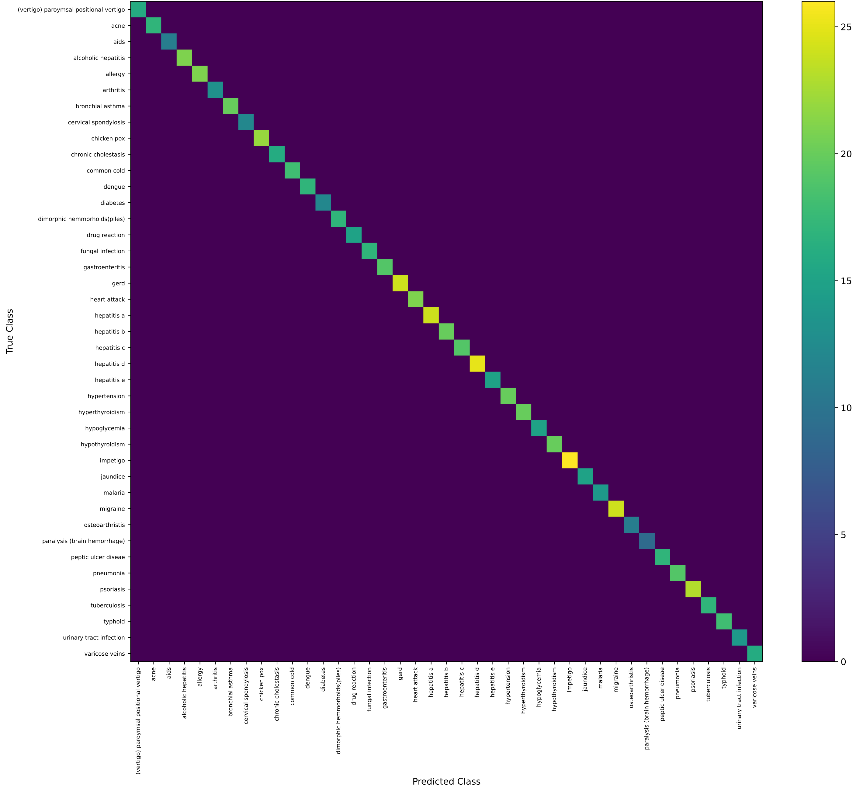
Figure 4.6: Confusion Matrix on the Test Set
