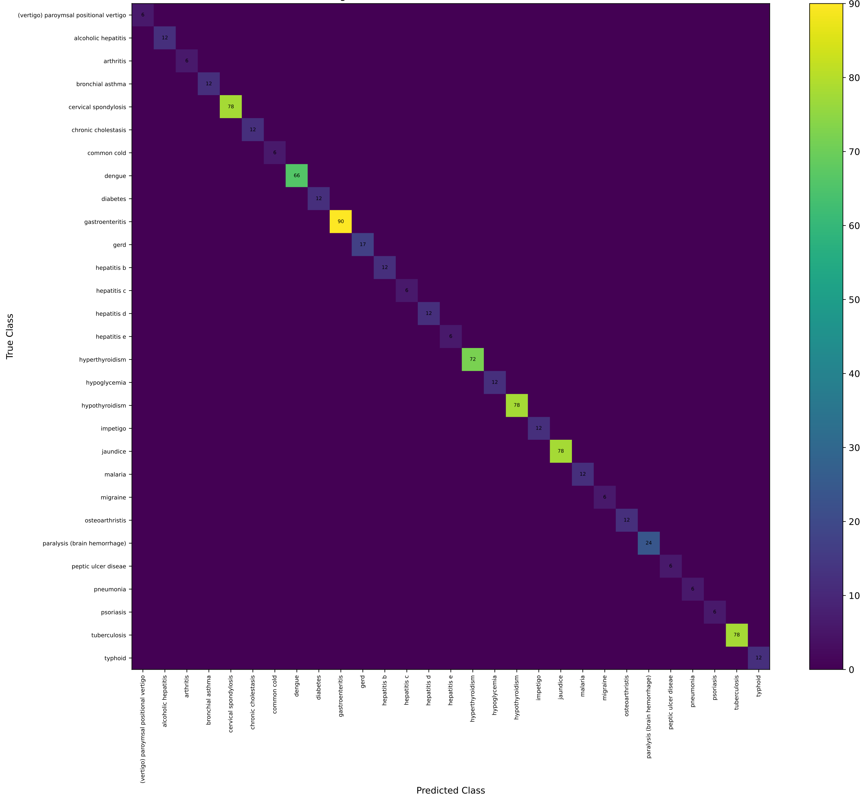
Figure 4.18: Confusion Matrix on the Test Set
