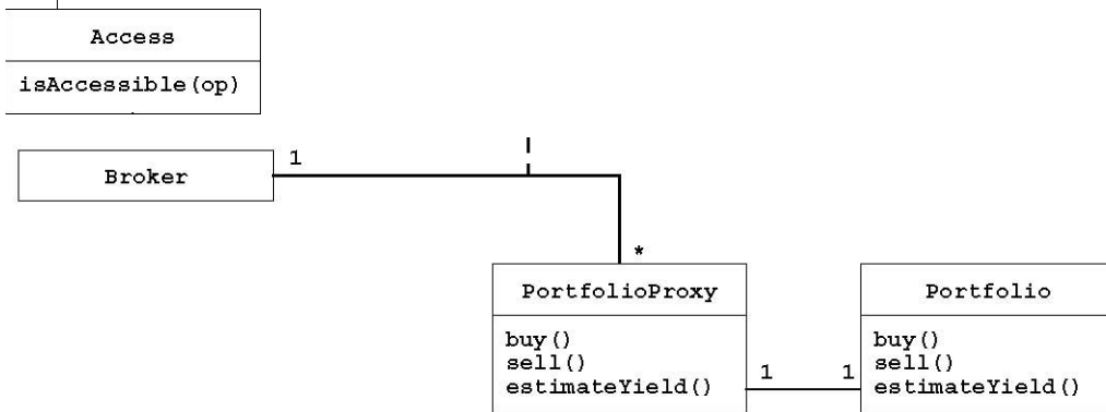
Figure 6-38 Dynamic access implemented with a protection Proxy. The Access association class contains a set of operations that Broker can use to access a Portfolio . Every operation in the PortfolioProxy first checks with the isAccessible() operation if the invoking Broker has legitimate access. Once access has been granted, PortfolioProxy delegates the operation to the actual Portfolio object. One Access association can be used to control access to many Portfolios .
