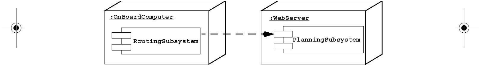
Figure 6-31 Allocation of MyTrip subsystems to hardware (UML deployment diagram). RoutingSubsystem runs on the OnBoardComputer while PlanningSubsystem runs on a WebServer.
