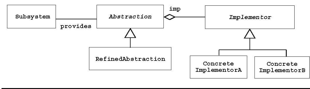
Figure 6-36 Bridge pattern (UML class diagram).
