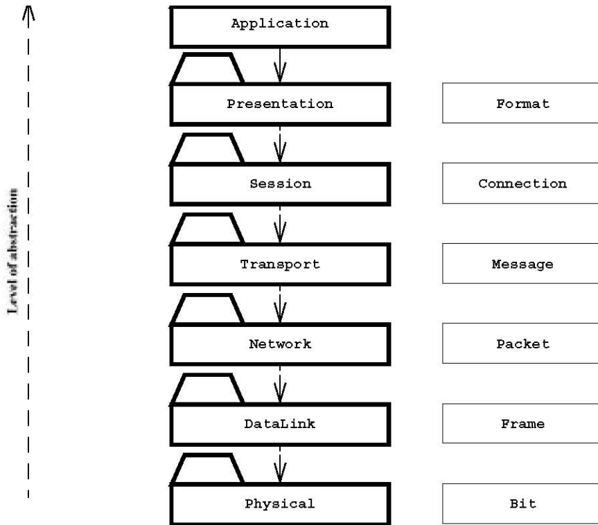
Figure 6-10 An example of closed architecture: the OSI model (UML class diagram). The OSI model decomposes network services into seven layers, each responsible for a different level of abstraction.
