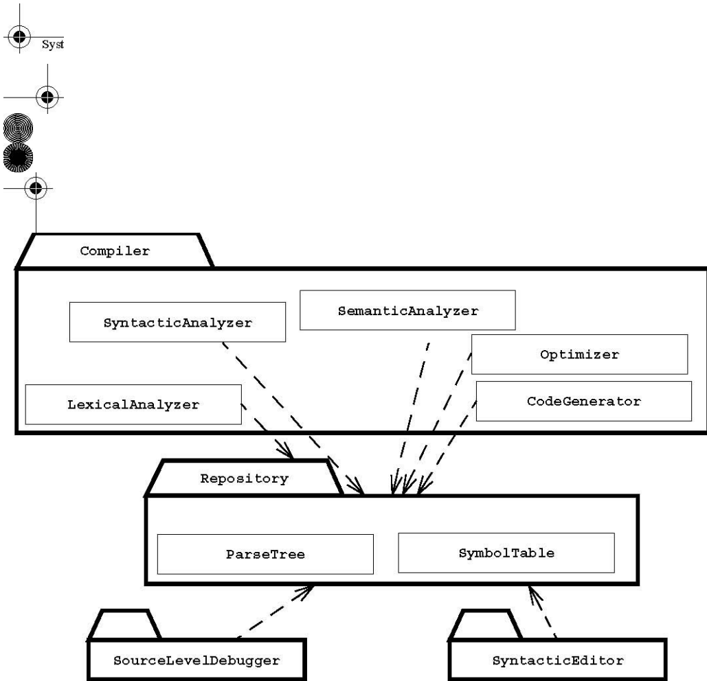
Figure 6-14 An instance of the repository architecture (UML Class diagram). A modern compiler incrementally generates a parse tree and a symbol table that can be later used by debuggers and syntax editors.
