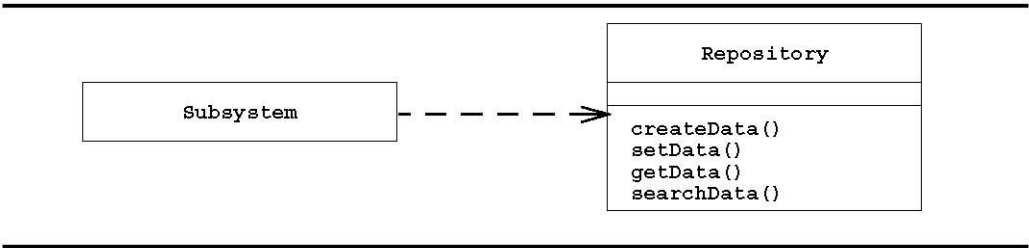
Figure 6-13 Repository architecture (UML class diagram). Every subsystem depends only on a central data structure called the repository. The repository in turn, has no knowledge of the other subsystems.
