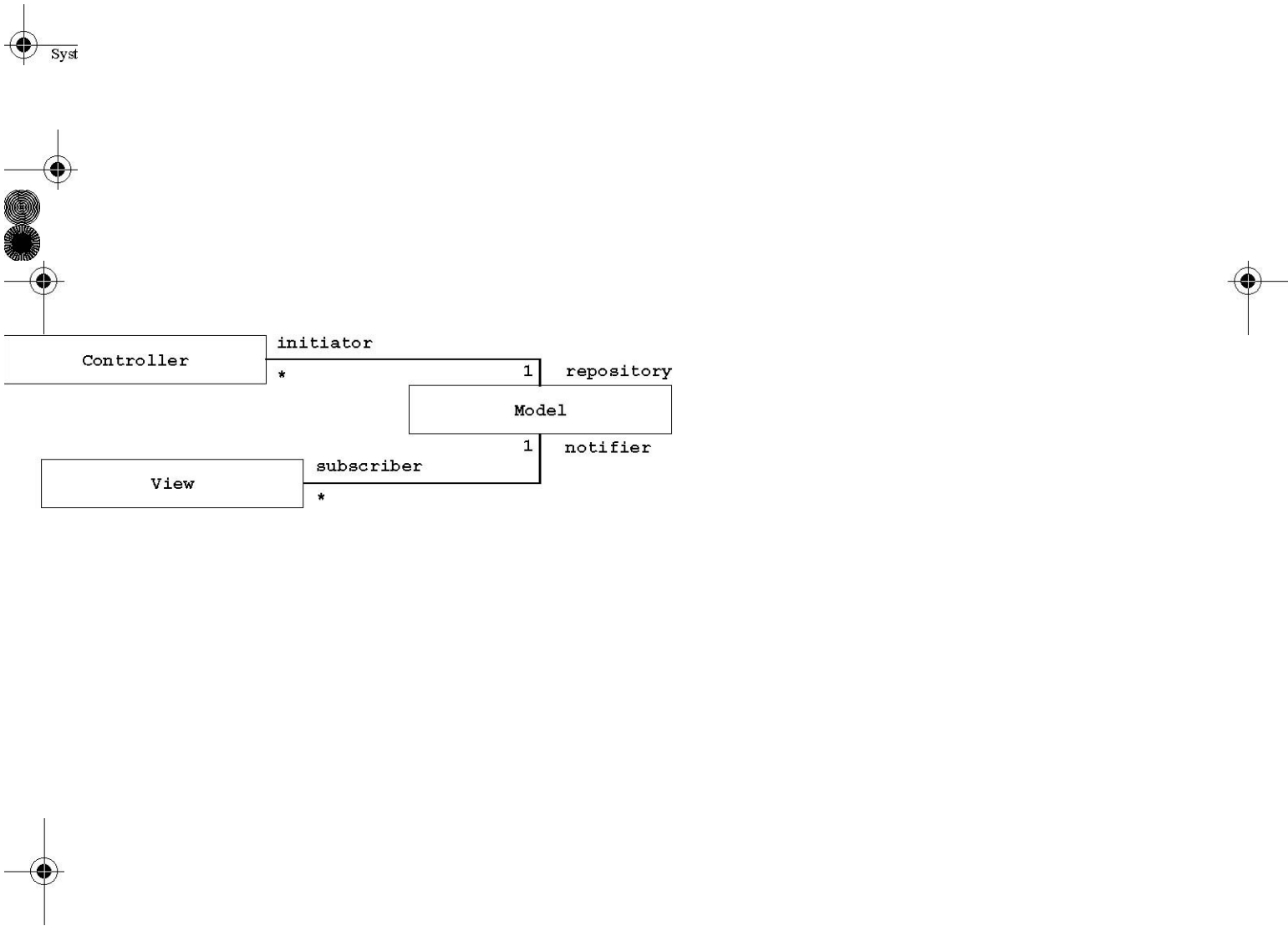
Figure 6-15 Model/View/Controller architecture (UML class diagram). The Controller gathers input from the user and sends messages to the Model. The Model maintains the central data structure. The View(s) display the Model and is notified (via a subscribe/notify protocol) whenever the Model is changed.
