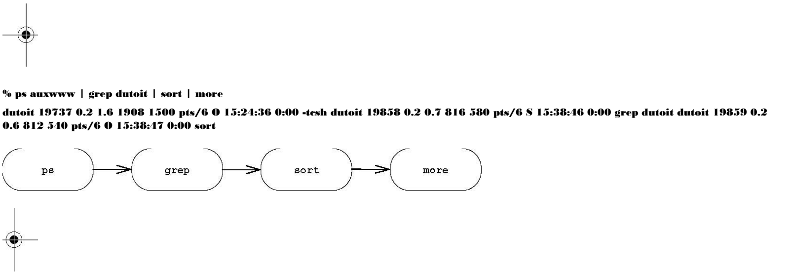
Figure 6-23 An instance of the pipe and filter architecture (Unix command and UML activity diagram).
