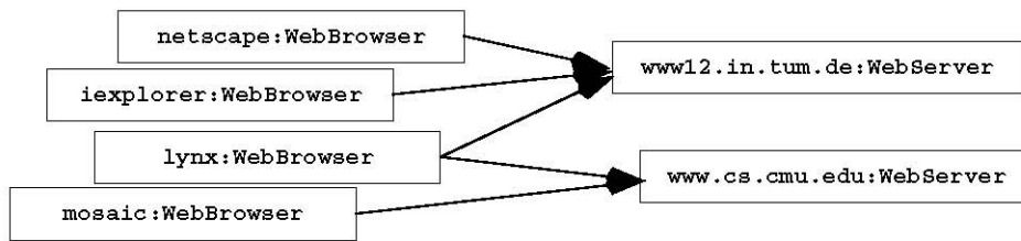
Figure 6-19 The World Wide Web as an instance of the client/server architecture (UML object diagram).
