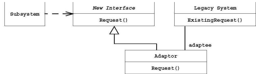
Figure 6-33 Adapter pattern (UML class diagram). The Adapter pattern is used to provide a different interface ( New Interface ) to an existing component ( Legacy System ).
