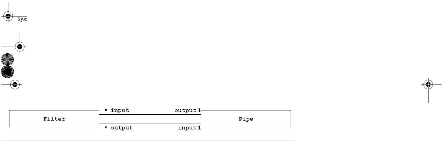
Figure 6-22 Pipe and filter architecture (UML class diagram). A Filter can have many inputs and outputs. A Pipe connects one of the outputs of a Filter to one of the inputs of another Filter .
