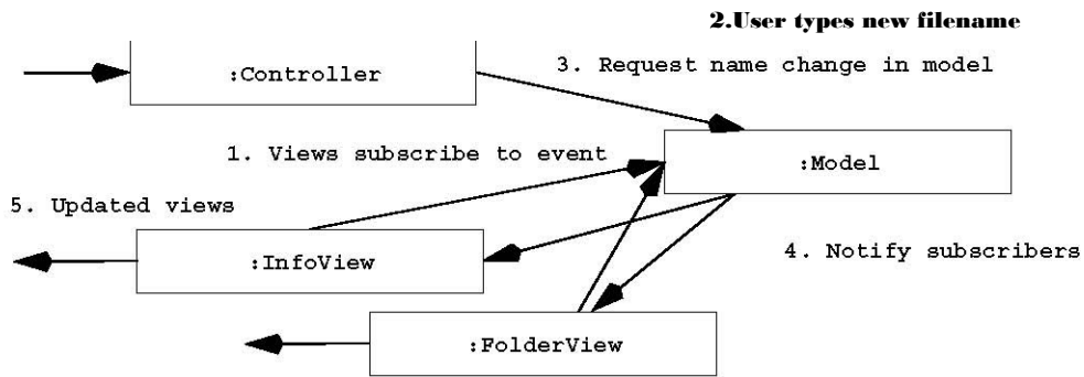
Figure 6-16 Sequence of events in the Model/View/Control architecture (UML collaboration diagram).
