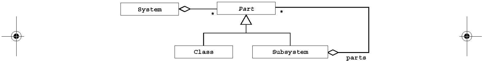
Figure 6-3 Subsystem decomposition (UML class diagram).
