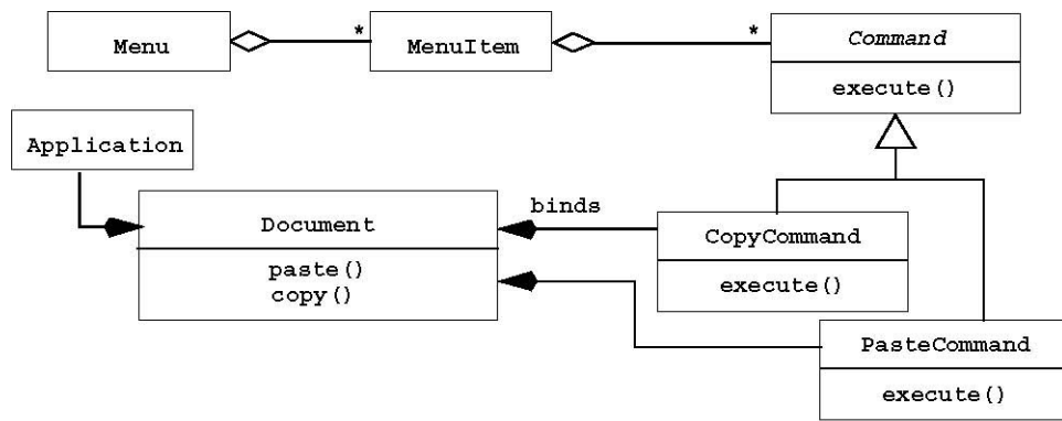
Figure 6-45 An example of a Command pattern (UML class diagram). In this example, menu items and operations on documents are decoupled. This enables us to centralize control flow in the command objects (CopyCommand and PasteCommand) instead of spreading it across boundary objects (MenuItem) and entity objects (Document).
