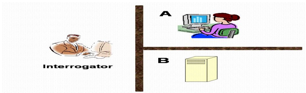
Turing Test
