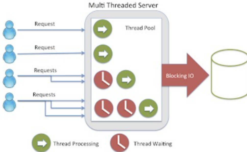
Figure 2.1 - Multithreaded Server
