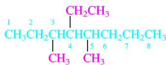
4-ethyl-3,5-dimethyloctane.
