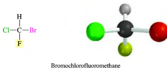
Bromochlorofluoromethane
