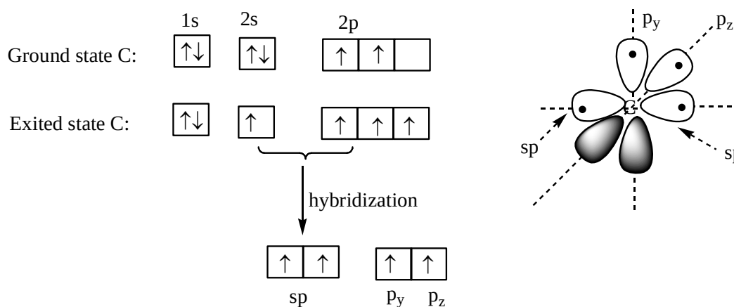
Figure 1.10 Mixing the s orbital with the one p orbitals generates two sp hybrid orbitals. The hybrid orbital indicates the presence of two unhybridized p orbitals that can overlap side-to-side. As a result two \pi bonds produced.
