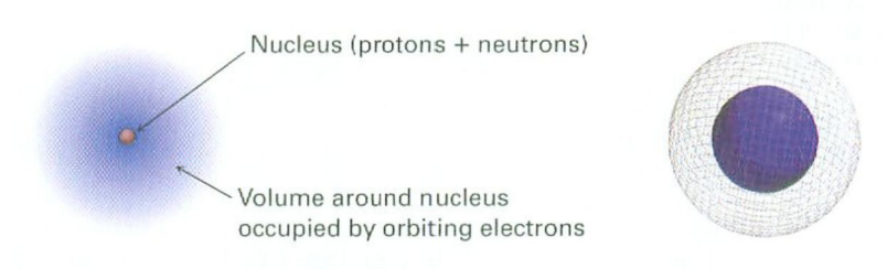
Figure 1.1 A schematic view of an atom
