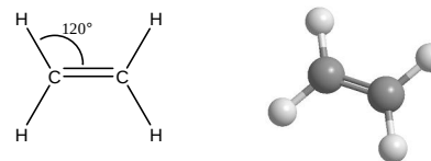
Figure 1.9 The structure of Ethene. orbital overlap of two sp^2 hybrid carbon forms double bond
