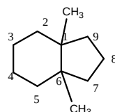
1,6-dimethylbicyclo[4,3,0]nonane
