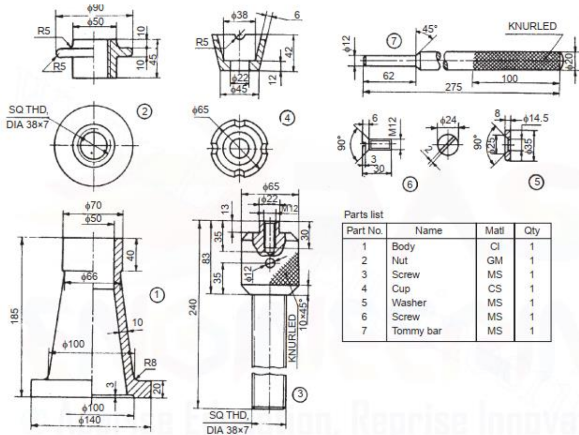
Fig. 18.51 Screw jack
