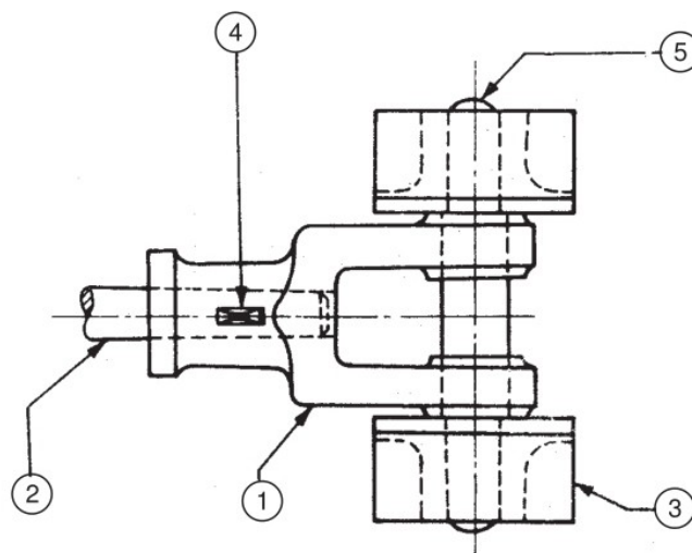
Fig. 18.2A Steam engine crosshead
