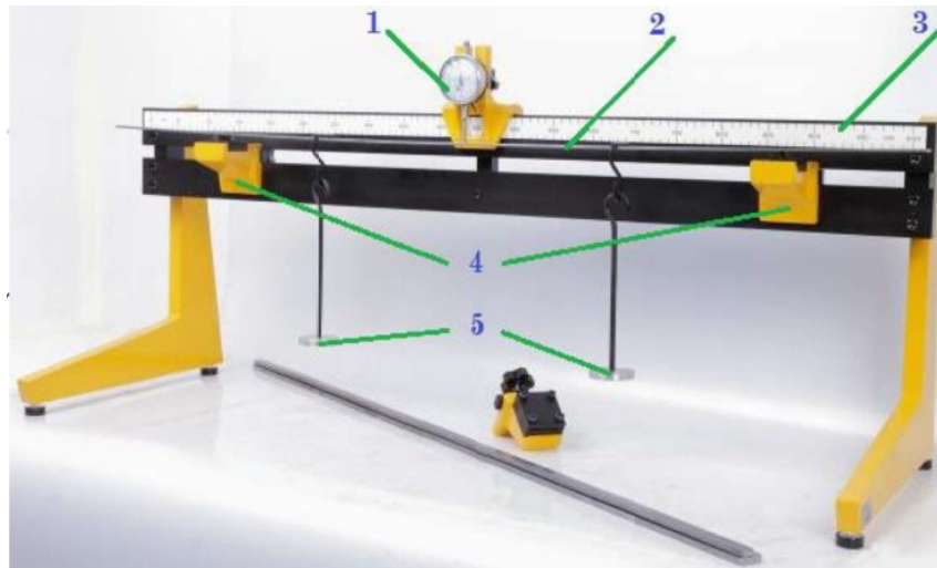
Figure 7: beam deflection equipment
