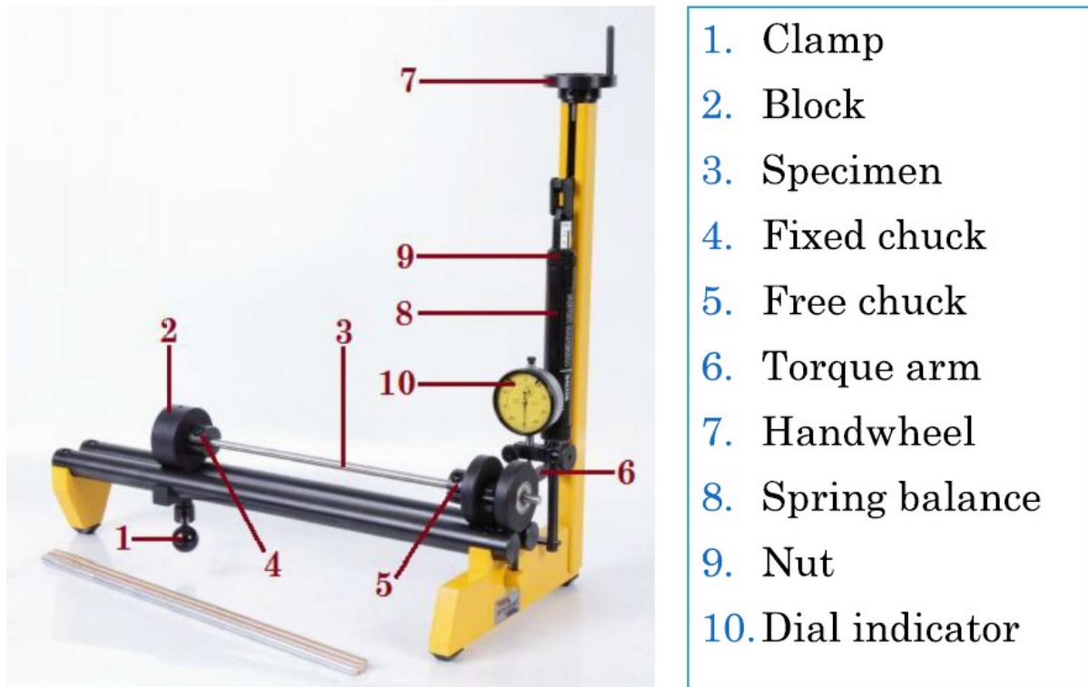
Figure 16: torsion of beam equipment
