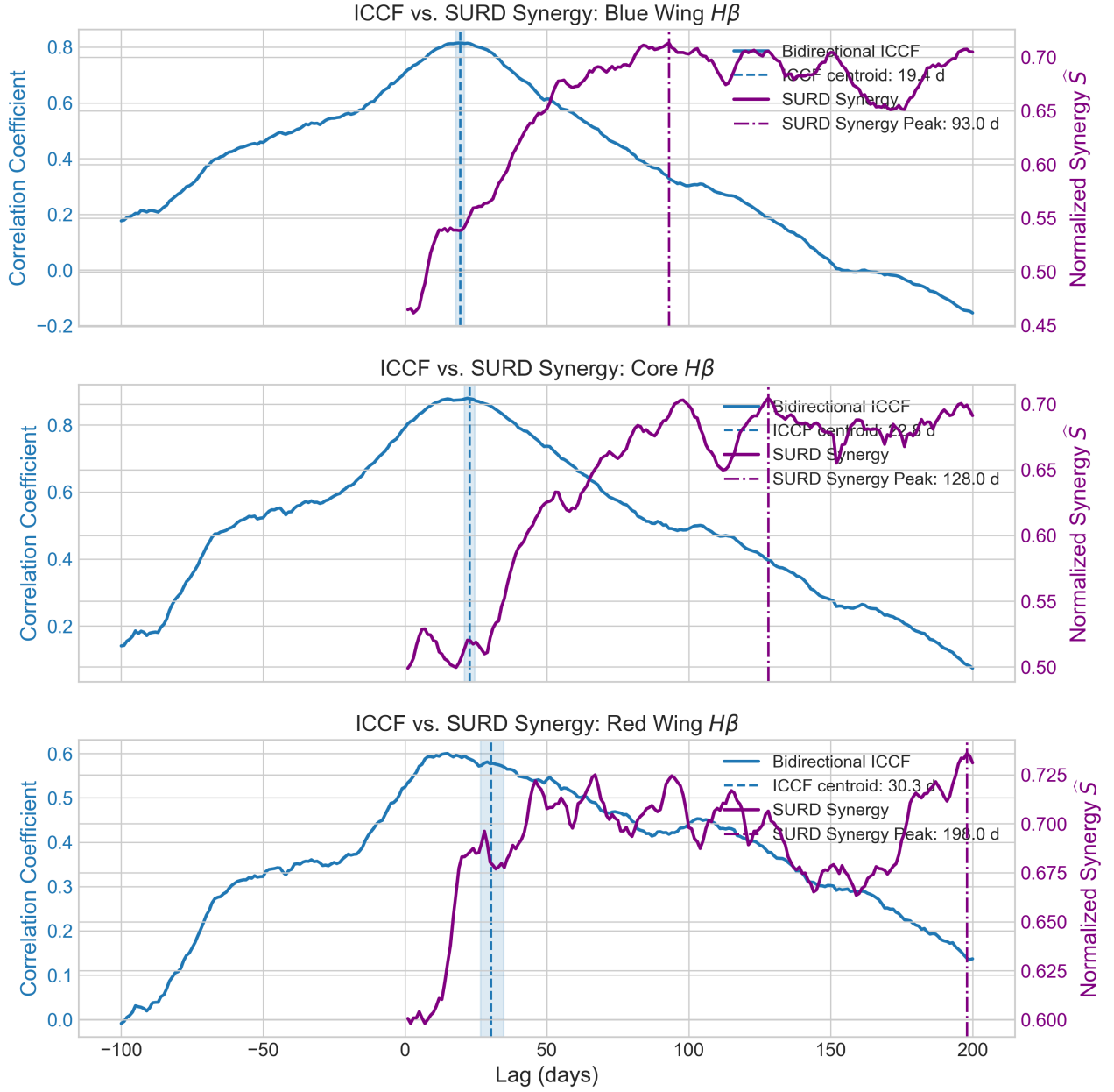
Figure 4. Native-cadence bidirectional ICCF (blue) and normalized three-predictor SURD total synergy (purple). Blue dashed lines and bands show the FR/RSS centroid median and 16th–84th percentiles; purple dash-dotted lines mark the descriptive SURD maxima. The quantities have different estimands and the SURD maxima are globally non-significant.
