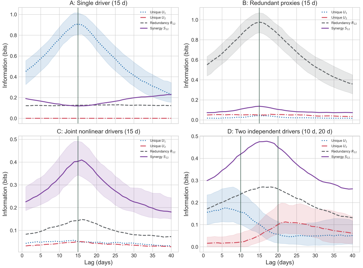
Figure 7. Median SURD decompositions over 100 synthetic realizations sampled under the NGC 5548 observing footprint. Shading spans the 16th–84th percentiles for the designated diagnostic atom (two atoms in Case 4); vertical lines mark the true delays. Cases 1–3 recover their isolated generating mechanisms, whereas the additive two-delay stress test is dominated by broad synergy and redundancy.
