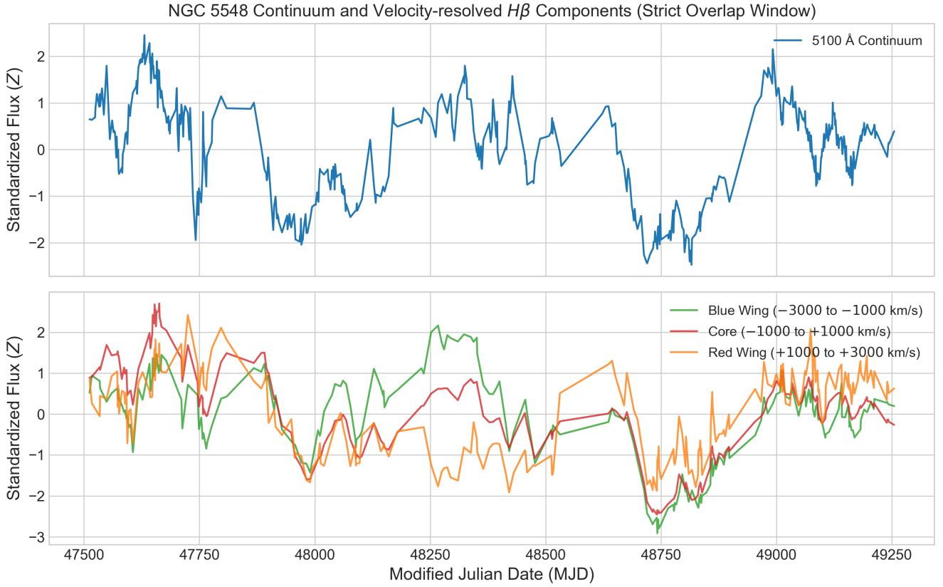
Figure 1. Top panel: Standardized 5100 Å continuum light curve for NGC 5548 over the strictly aligned overlap window (JD less 2400000: 47512–49255). Bottom panel: Standardized velocity-resolved H \beta components (Blue Wing, Line Core, and Red Wing) resampled onto the shared 1.0-day grid.
