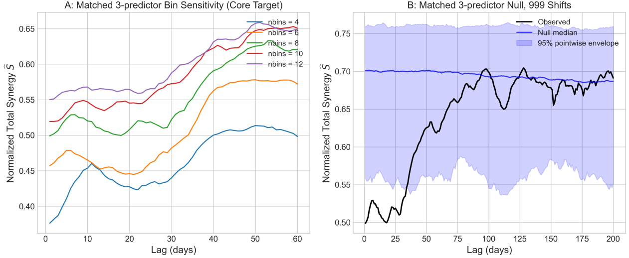
Figure 3. Matched three-predictor robustness checks for the core target. Panel A varies the equal-width histogram from 4 to 12 bins over 1–60 d. Panel B compares the observed normalized total synergy with the median and pointwise 95% envelope from 999 circular-shift realizations. The global test uses each realization’s maximum over the full 1–200 d scan rather than this pointwise envelope.
