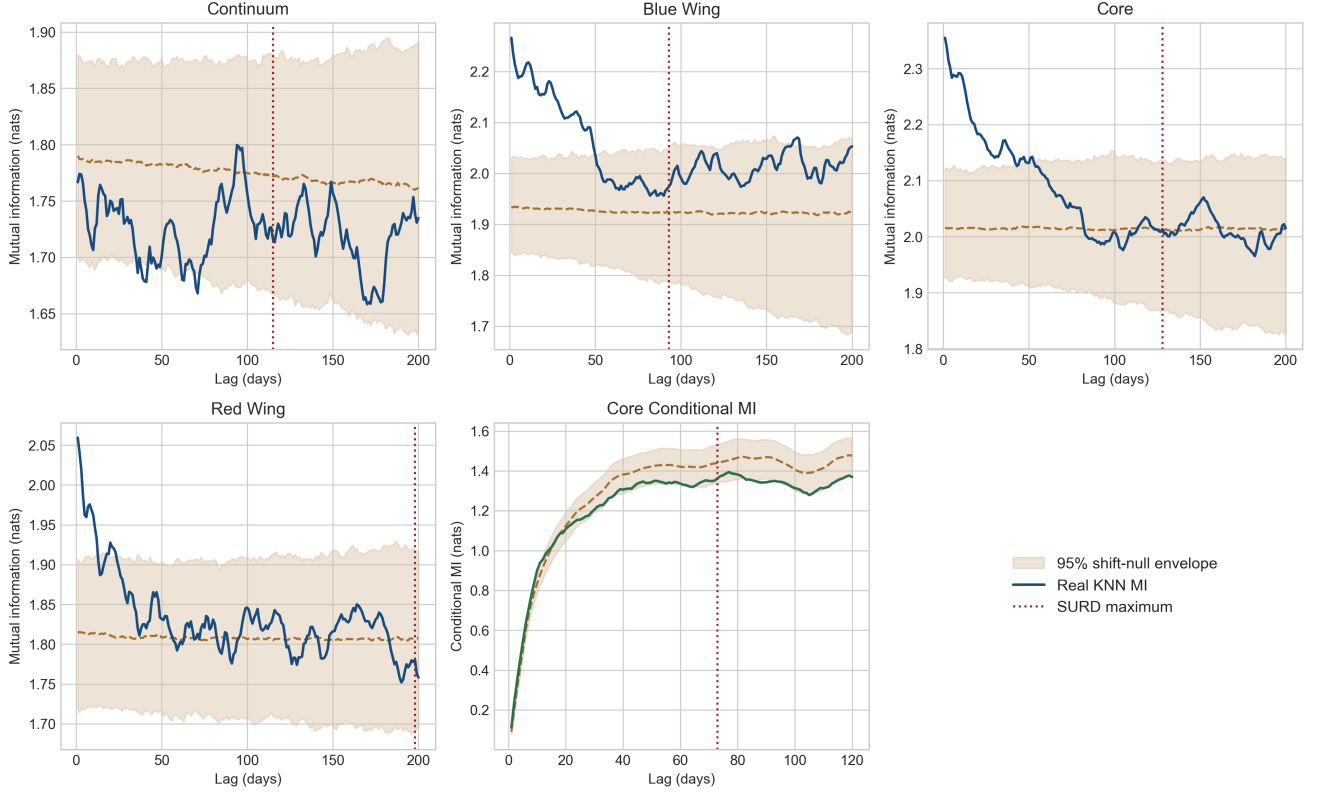
Figure 11. KNN mutual-information cross-check for k = 5 . Blue or green curves show the real total or conditional mutual information, tan bands show pointwise 95% circular-shift envelopes, and dotted red lines mark the corresponding histogram-SURD maxima. Prompt dependence is visible for the three line targets, whereas the long-lag SURD maxima and the conditioned 73-day maximum lie within their null distributions.
