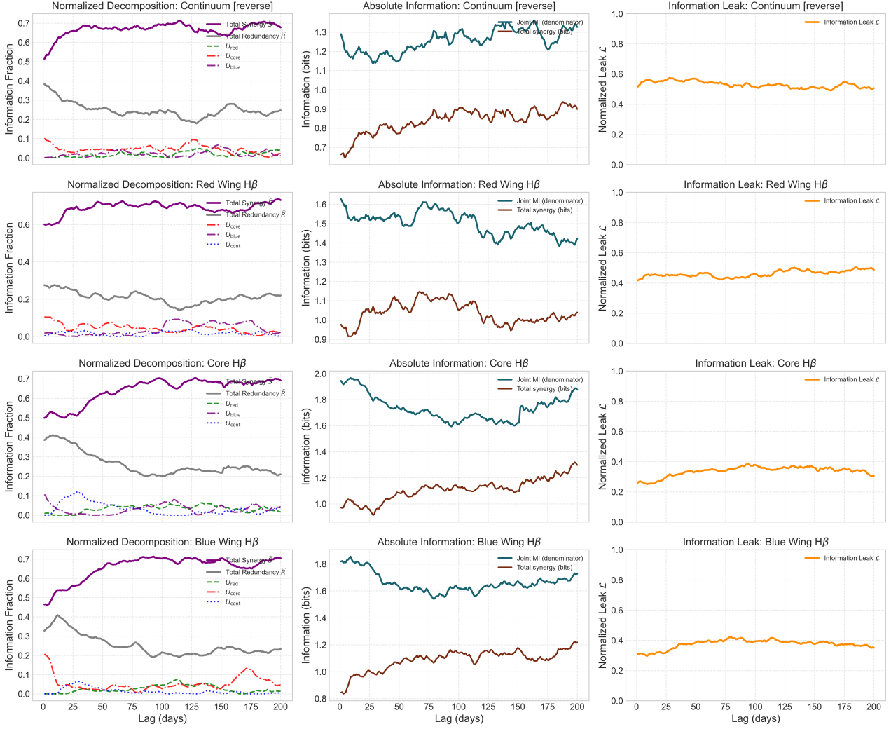
Figure 2. Three-predictor round-robin scans. The left column shows normalized atoms, which sum to unity. The middle column shows total joint mutual information, the normalization denominator, together with absolute total synergy in bits. The right column shows normalized information leak \mathcal{L} = H(Y | X_1, X_2, X_3)/H(Y) . Total synergy is S_{12} + S_{13} + S_{23} + S_{123} , with an analogous sum for redundancy. The continuum-target row is a reverse-prediction estimator diagnostic, not a physical line-to-continuum reverberation model.
