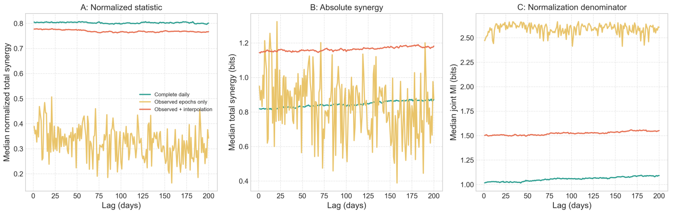
Figure 8. Matched three-predictor negative-control ablation over 200 independent red-noise realizations. Curves show medians for complete daily data, exact observed epochs, and observed epochs followed by daily interpolation. The panels separate normalized total synergy, absolute total synergy, and its joint-MI normalization denominator. The observed-only estimate is shown diagnostically but is severely undersampled.
