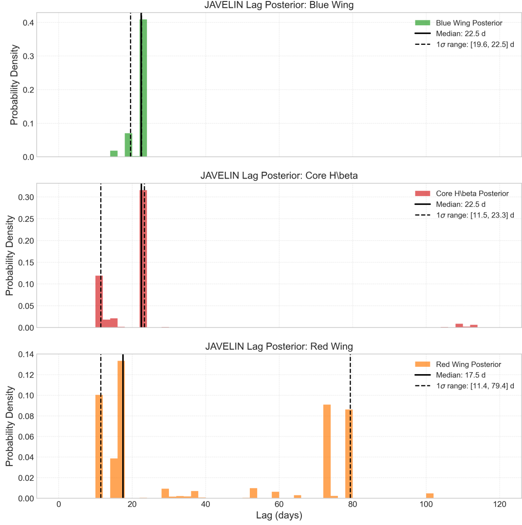
Figure A1. Archived JAVELIN lag-chain histograms. The multimodal chains are shown for transparency only and are not used for inference.
