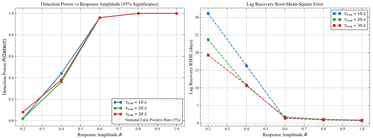
Figure 5. Detection power (left) and lag recovery root-mean-square error (right) as a function of response amplitude A across delays \tau_{\text{true}} \in \{10, 20, 30\} d. Dotted horizontal line marks the nominal 5% false positive rate under the null ( A = 0.0 ). A coherent response amplitude A \geq 0.5 – 0.6 is required to achieve \geq 90\% detection power and lag RMSE < 2.0 d under the NGC 5548 observing cadence.
