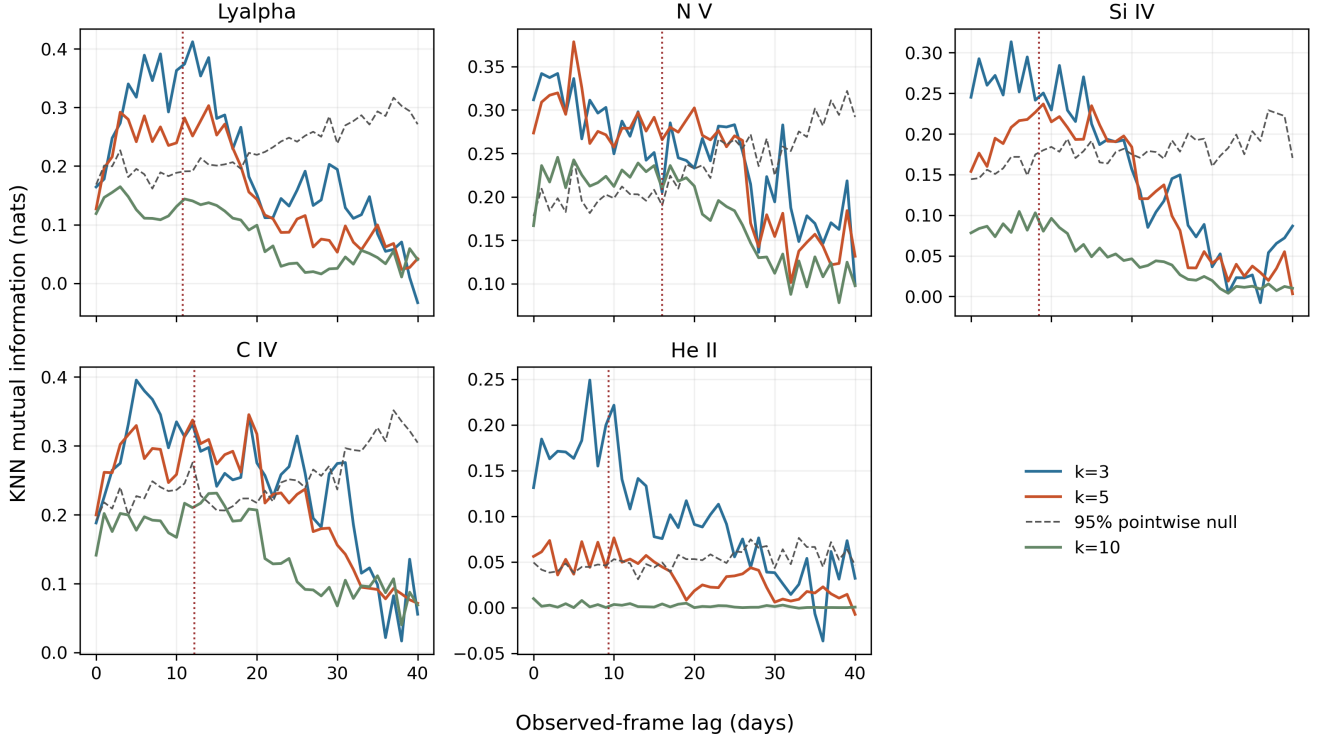
Figure 12. Native-cadence KNN mutual-information scans for Mrk 817. Coloured curves show k = 3, 5 , and 10 ; grey dashed curves are the pointwise 95% circular-shift envelopes for k = 5 ; dotted red lines mark the observed-frame equivalents of the published delays. Pointwise excursions are not equivalent to the scan-wide tests in Table 11.
