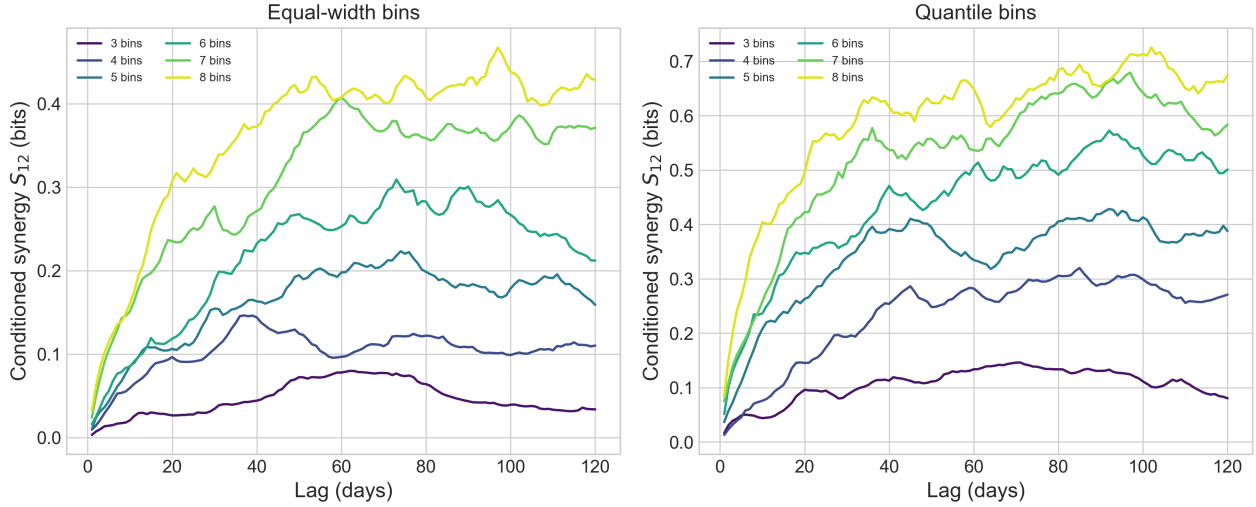
Figure 10. History-conditioned core-target synergy over 1–120 d for 3–8 equal-width bins (left) and quantile bins (right). Both peak amplitude and peak location vary with discretization; increasing the number of bins systematically inflates the estimated synergy as occupancy declines.
