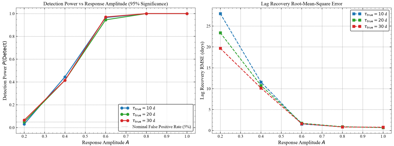
Figure 5. Detection power and lag RMSE as a function of the linear mixing coefficient A . At A = 0.6 , power ranges from 0.945 to 0.970, while its 95% Wilson lower bounds range from 0.904 to 0.936.
