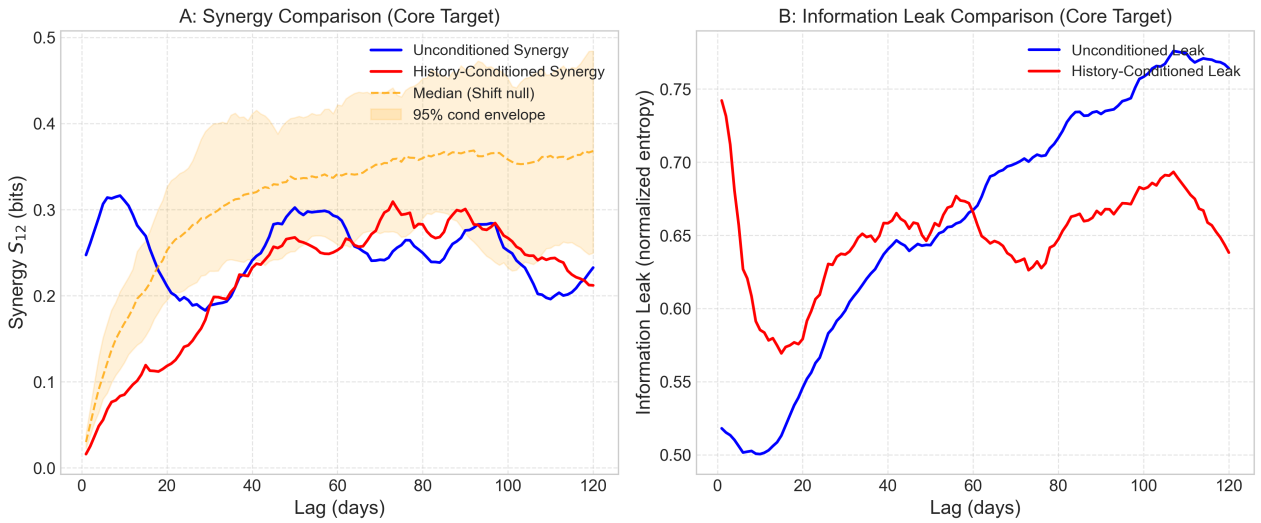
Figure 10. Comparison of the unconditioned (blue) and target-history conditioned (red) SURD synergy (left) and information leak (right) curves for the Core H \beta target over the 1–120 d window for which conditional surrogates were computed. The orange shaded band and dashed line represent the pointwise 95% circular-shift surrogate envelope and median at each lag for the conditioned scan. The global max-statistic test compares the observed peak to the distribution of per-realization surrogate maxima (whose median is 0.4043 bits, with the 95th percentile higher) and is not represented by a single pointwise threshold curve. Within this tested window, conditioning on the target’s own past shifts the local synergy peak to 73 days, but the peak is statistically insignificant ( p_{\text{global}} = 0.9802 ) under this null and does not establish physical coupling.
