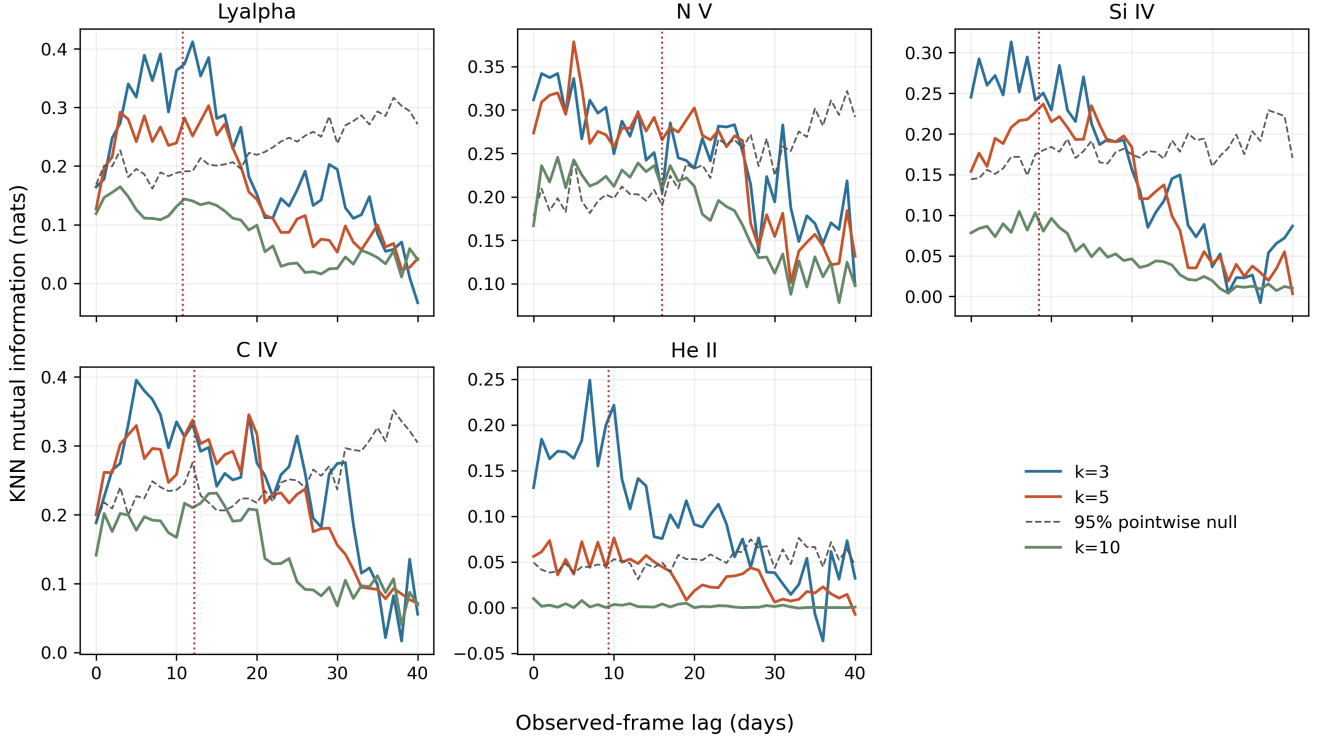
Figure 13. Native-cadence KNN mutual-information scans for Mrk 817. Coloured curves show k = 3, 5 , and 10 ; grey dashed curves are the pointwise 95% circular-shift envelopes for k = 5 ; dotted red lines mark the observed-frame equivalents of the published delays. Pointwise excursions are not equivalent to the scan-wide tests in Table 11.
