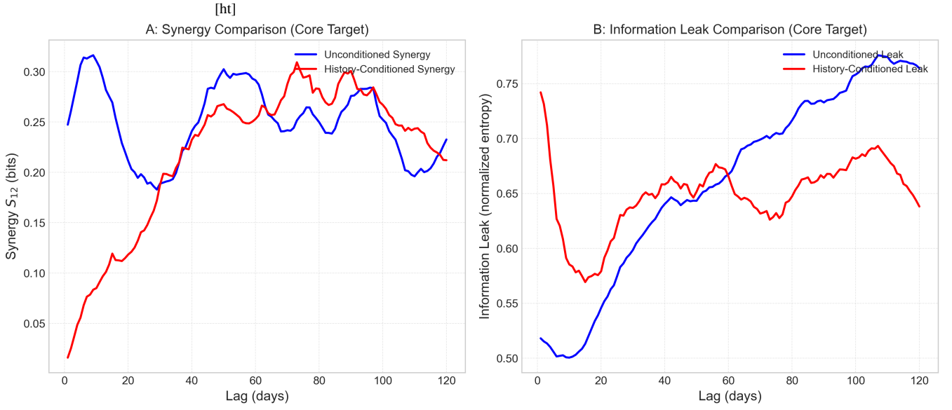
Figure 7. Comparison of the unconditioned (blue) and target-history conditioned (red) SURD synergy (left) and information leak (right) curves for the Core H \beta target. Conditioning on the target's own past shifts the synergy peak from a short autocorrelation-dominated delay of 9 days to a robust, long-term cross-component delay of 73 days.
