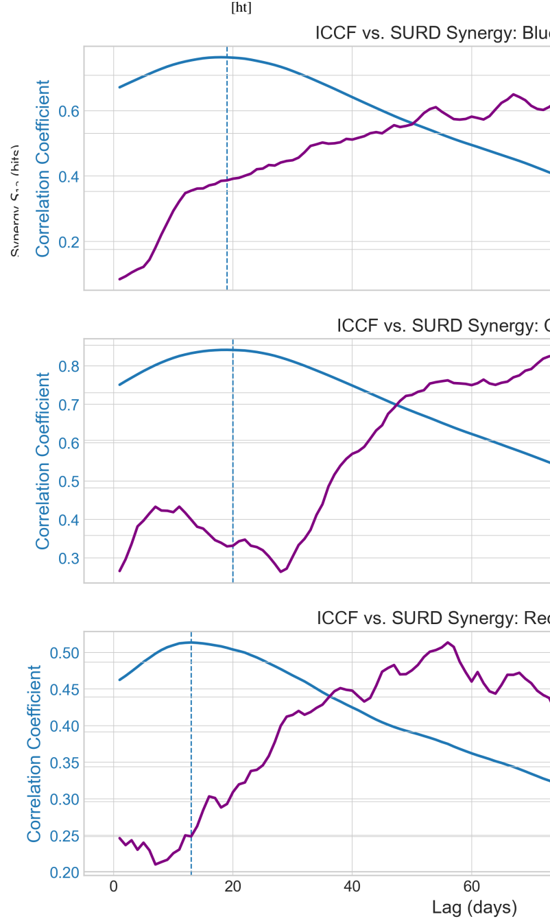
Figure 4. Comparison of the Inter-Correlation Function (ICCF, blue) and the SURD synergy curve (purple) for the Blue Wing (top), Core (middle), and Red Wing (bottom) targets. Vertical lines mark the respective peak lags.
