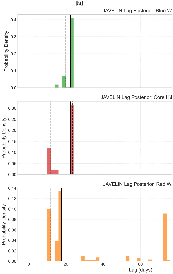
Figure 5. JAVELIN MCMC lag posterior distributions for the Blue Wing (top), Core (middle), and Red Wing (bottom) of H \beta in NGC 5548. Black solid and dashed lines represent the median and 1 \sigma (16th–84th percentiles) confidence intervals, respectively.
