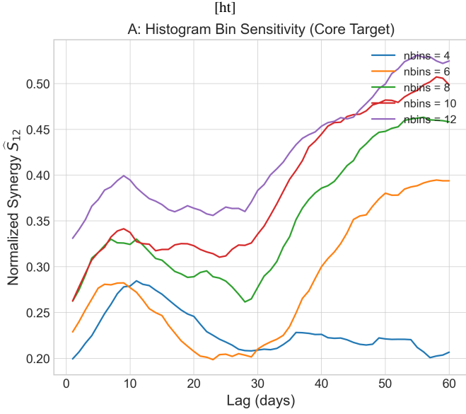
Figure 3. Panel A: Sensitivity of Core H \beta synergy to the number of histogram bins ( n_{\text{bins}} = 4, 6, 8, 10, 12 ) over lags 1–60 days, showing strong qualitative stability. Panel B: Real synergy curve for Core H \beta compared with the median and 95% percentile envelopes for circular-shift (blue) and block-bootstrap (red) surrogate runs, indicating local significance relative to standard nulls.
