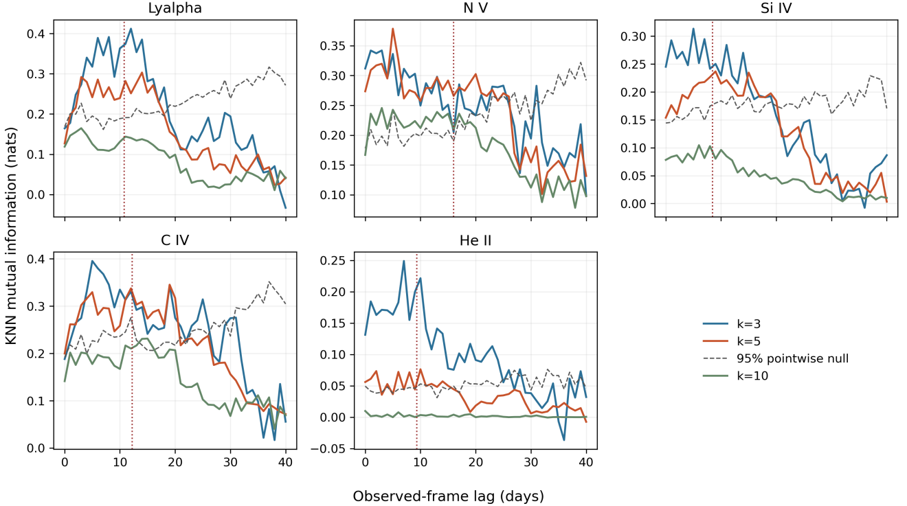
Figure 10. Native-cadence KNN mutual-information scans for Mrk 817. Coloured curves show k = 3, 5 , and 10 ; grey dashed curves are the pointwise 95% circular-shift envelopes for k = 5 ; dotted red lines mark the observed-frame equivalents of the published delays. Pointwise excursions are not equivalent to the scan-wide tests in Table 8.
