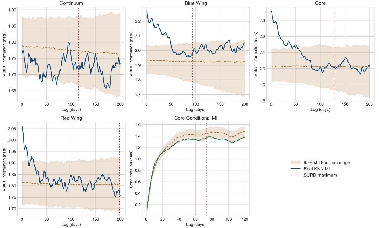
Figure 9. KNN mutual-information cross-check for k = 5 . Blue or green curves show the real total or conditional mutual information, tan bands show pointwise 95% circular-shift envelopes, and dotted red lines mark the corresponding histogram-SURD maxima. Prompt dependence is visible for the three line targets, whereas the long-lag SURD maxima and the conditioned 73-day maximum lie within their null distributions.
