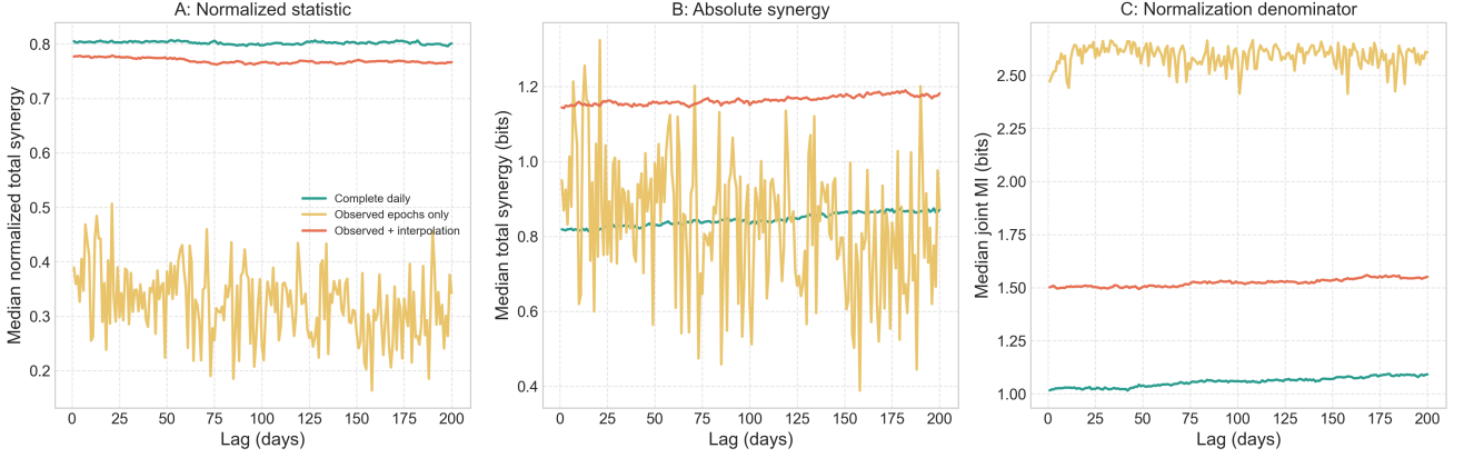
Figure 6. Matched three-predictor negative-control ablation over 200 independent red-noise realizations. Curves show medians for complete daily data, exact observed epochs, and observed epochs followed by daily interpolation. The panels separate normalized total synergy, absolute total synergy, and its joint-MI normalization denominator. The observed-only estimate is shown diagnostically but is severely undersampled.
