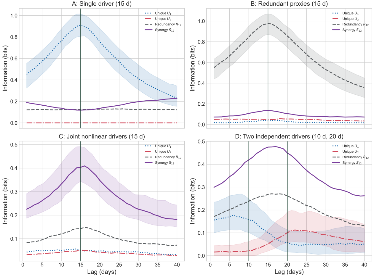
Figure 5. Median SURD decompositions over 100 synthetic realizations sampled under the NGC 5548 observing footprint. Shading spans the 16th–84th percentiles for the designated diagnostic atom (two atoms in Case 4); vertical lines mark the true delays. Cases 1–3 recover their isolated generating mechanisms, whereas the additive two-delay stress test is dominated by broad synergy and redundancy.
