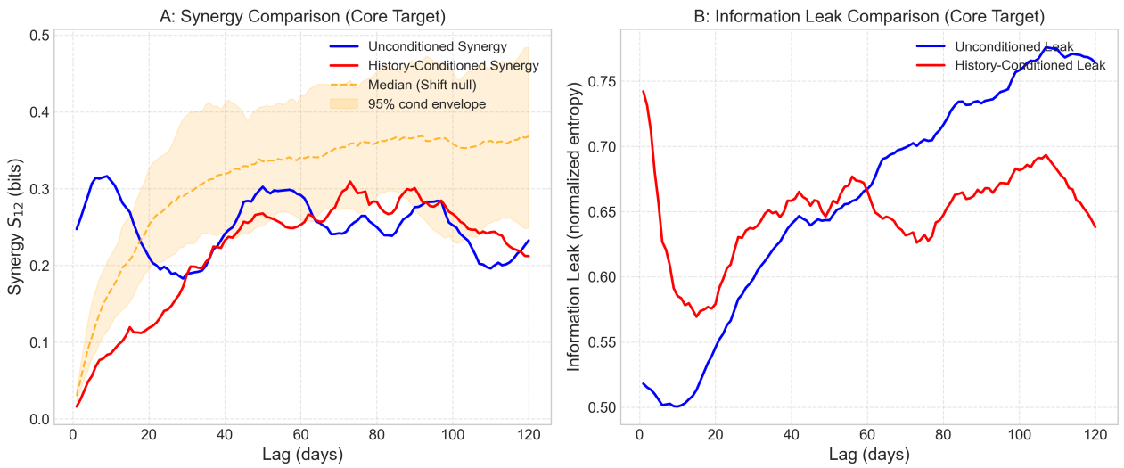
Figure 7. Comparison of the unconditioned (blue) and target-history conditioned (red) SURD synergy (left) and information leak (right) curves for the Core H\beta target over the 1–120 d window for which conditional surrogates were computed. The orange shaded band and dashed line represent the pointwise 95% circular-shift surrogate envelope and median at each lag for the conditioned scan. The global max-statistic test compares the observed peak to the distribution of per-realization surrogate maxima (whose median is 0.4043 bits, with the 95th percentile higher) and is not represented by a single pointwise threshold curve. Within this tested window, conditioning on the target’s own past shifts the local synergy peak to 73 days, but the peak is statistically insignificant ( p_{\text{global}} = 0.9802 ) under this null and does not establish physical coupling.
