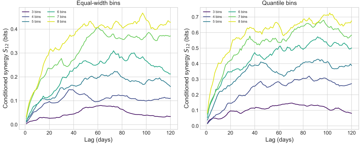
Figure 8. History-conditioned core-target synergy over 1–120 d for 3–8 equal-width bins (left) and quantile bins (right). Both peak amplitude and peak location vary with discretization; increasing the number of bins systematically inflates the estimated synergy as occupancy declines.
