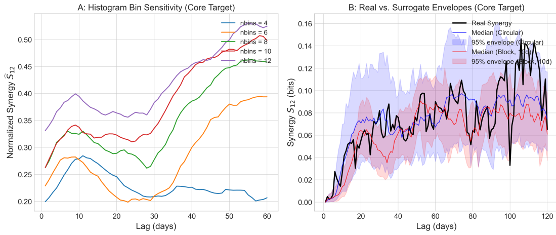
Figure 3: Panel A: Sensitivity of Core H \beta synergy to the number of histogram bins ( n_{\text{bins}} = 4, 6, 8, 10, 12 ) over lags 1–60 days, showing strong qualitative stability. Panel B: Real synergy curve for Core H \beta compared with the median and 95% percentile envelopes for circular-shift (blue) and block-bootstrap (red) surrogate runs, indicating local significance relative to standard nulls.
