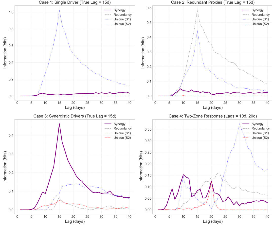
Figure 6: SURD information decomposition scans for the four synthetic benchmark cases: Case 1 (Single Driver), Case 2 (Redundant Proxies), Case 3 (Synergistic Drivers), and Case 4 (Two-Zone Response). Curves represent Synergy (purple), Redundancy (gray dashed), and Unique information for drivers S1 (blue dotted) and S2 (red dash-dot).
