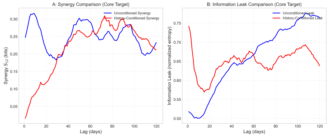
Figure 7: Comparison of the unconditioned (blue) and target-history conditioned (red) SURD synergy (left) and information leak (right) curves for the Core H\beta target. Conditioning on the target's own past shifts the synergy peak from a short autocorrelation-dominated delay of 9 days to a robust, long-term cross-component delay of 73 days.
