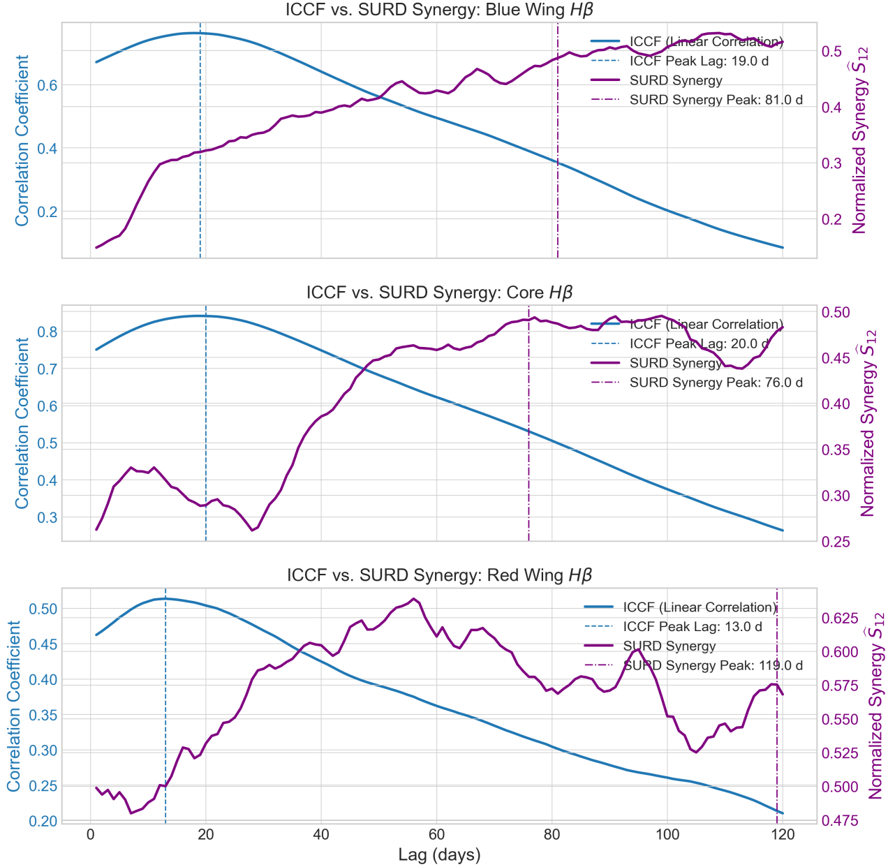
Figure 4. Comparison of the Inter-Correlation Function (ICCF, blue) and the SURD synergy curve (purple) for the Blue Wing (top), Core (middle), and Red Wing (bottom) targets. Vertical lines mark the respective peak lags.
