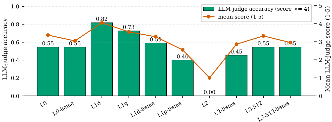
Per-variant LLM-judge accuracy (gpt-4o-mini grading)
