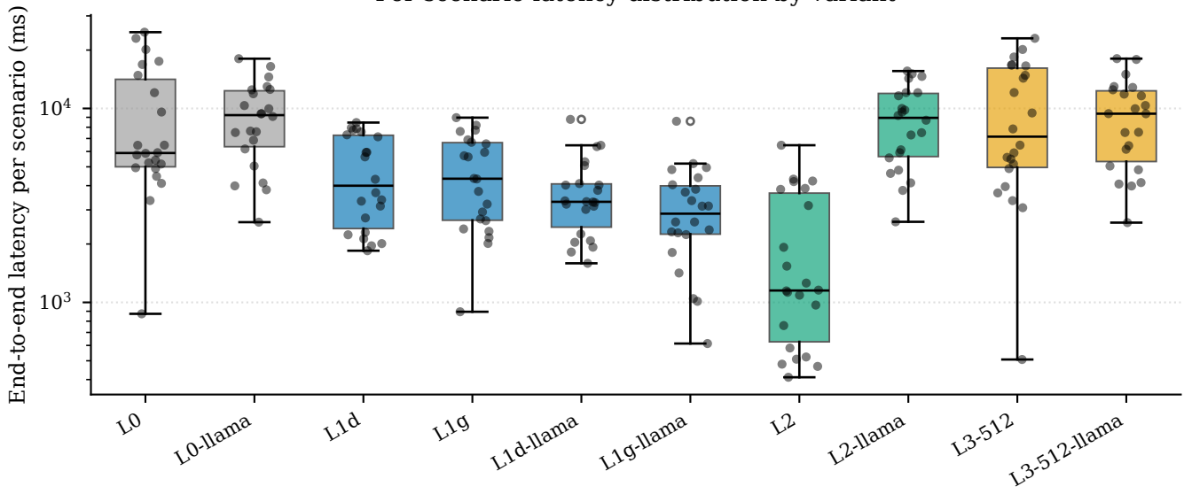
Per-scenario latency distribution by variant
