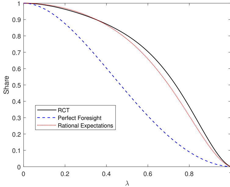
Figure 7: Share of transmission from a m_{t+1} news shock to \pi_t due to the adjustment of inflation expectations, comparing RCT estimates to benchmarks
