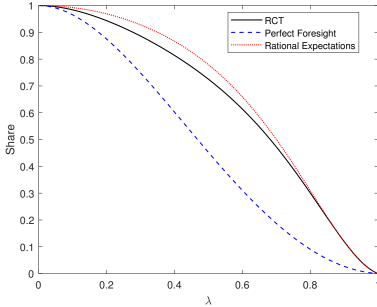
Figure 6: Share of transmission from a mc_{t+1} news shock to \pi_t due to the adjustment of inflation expectations, comparing RCT estimates to benchmarks
