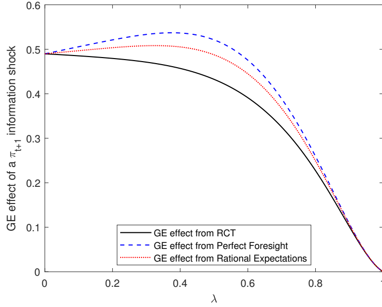
Figure 8: General equilibrium effects of a shock to s_{\pi_{t+1}} , comparing RCT estimates to alternatives with general equilibrium effects from other benchmarks
