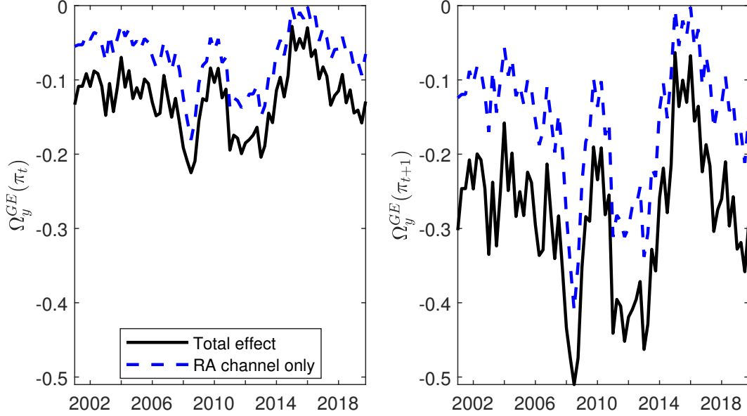
Figure 5: The causal effect of inflation perceptions \bar{E}_t \pi_t and expectations \bar{E}_t \pi_{t+1} on output y_t over time.
