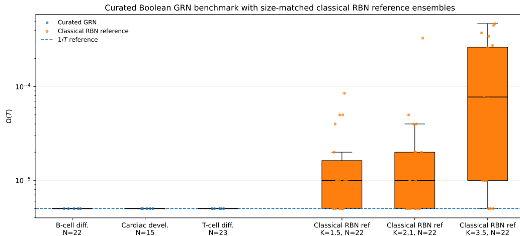
Figure 25: Curated Boolean GRN benchmark with size-matched classical RBN reference ensembles. Distributions of \Omega computed on curated Boolean GRN models across seeds/initial conditions, together with three size-matched classical RBN reference ensembles at representative connectivities ( K = 1.5, 2.1, 3.5 ). The dashed line marks the 1/T baseline. The curated GRNs remain clustered near this scale, consistent with stable regulatory dynamics, while the classical RBN controls span a broader recurrence range. These reference ensembles are included as scale controls rather than as a phase-classification test.
