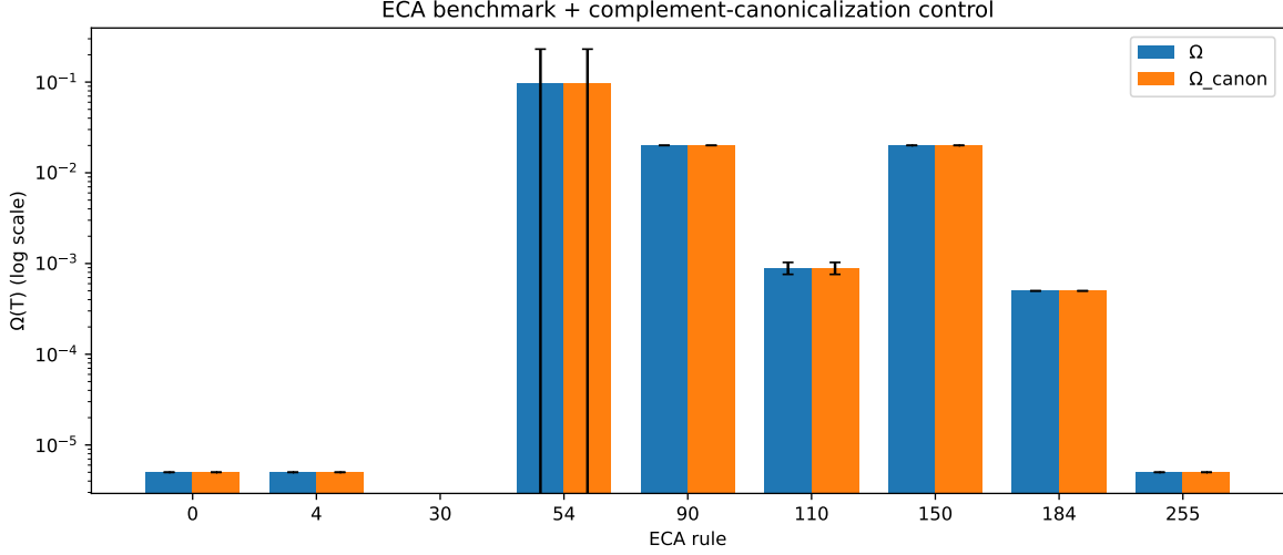
Figure 23: ECA benchmark and complement-symmetry control. Mean \Omega across seeds for a panel of classic ECA rules. Rule 54 attains the largest average value in this protocol, while additive Rules 90 and 150 also score highly because finite-ring linear dynamics generate exact recurrences. We also report \Omega_{\text{canon}} computed after canonicalizing each state under the complement quotient s \sim 1 - s (mapping to \min(s, 1 - s) ).
