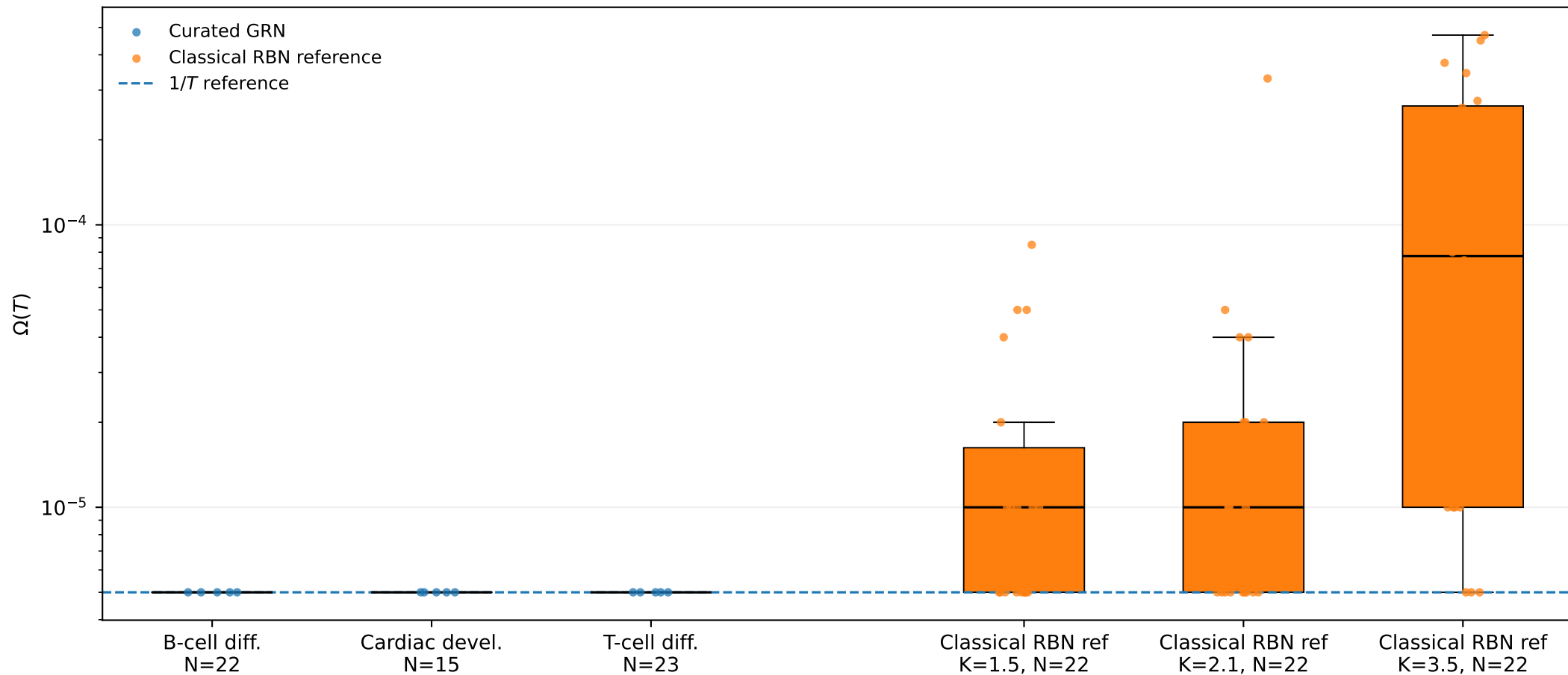
Curated Boolean GRN benchmark with size-matched classical RBN reference ensembles
