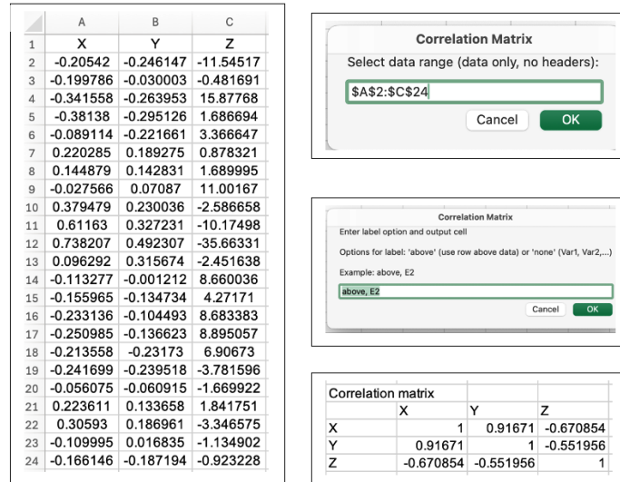
Figure 7: Correlation matrix
