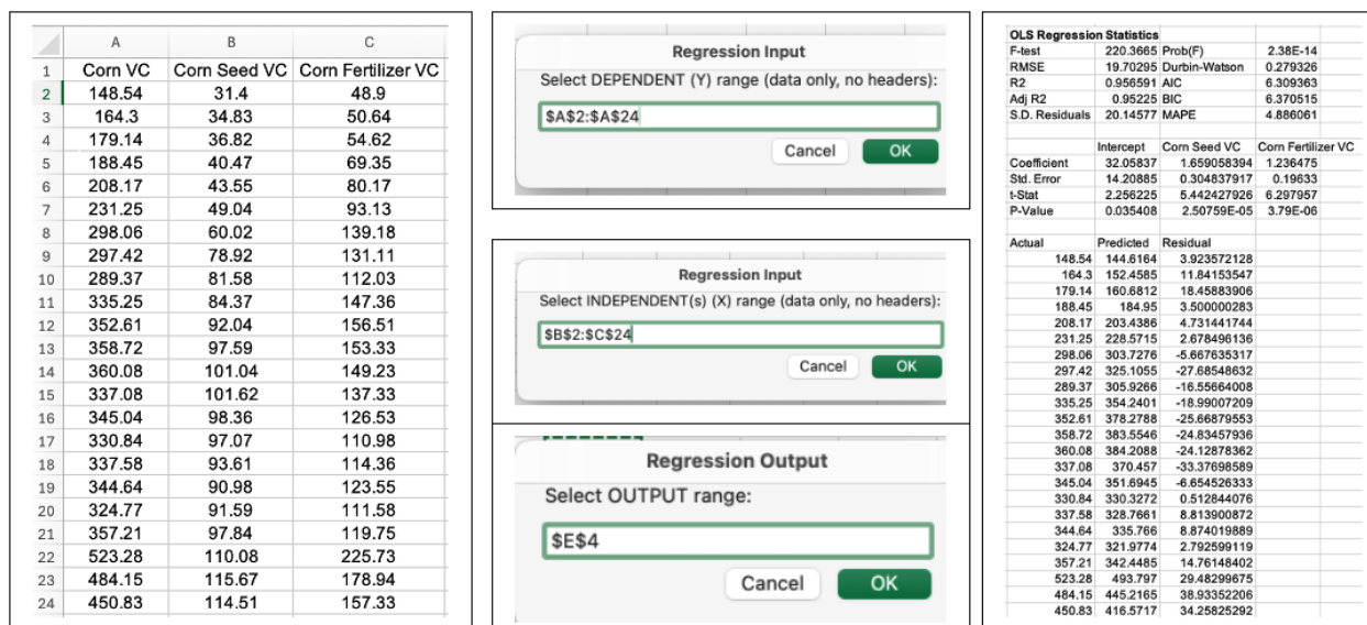
Figure 5: Regression Analysis
