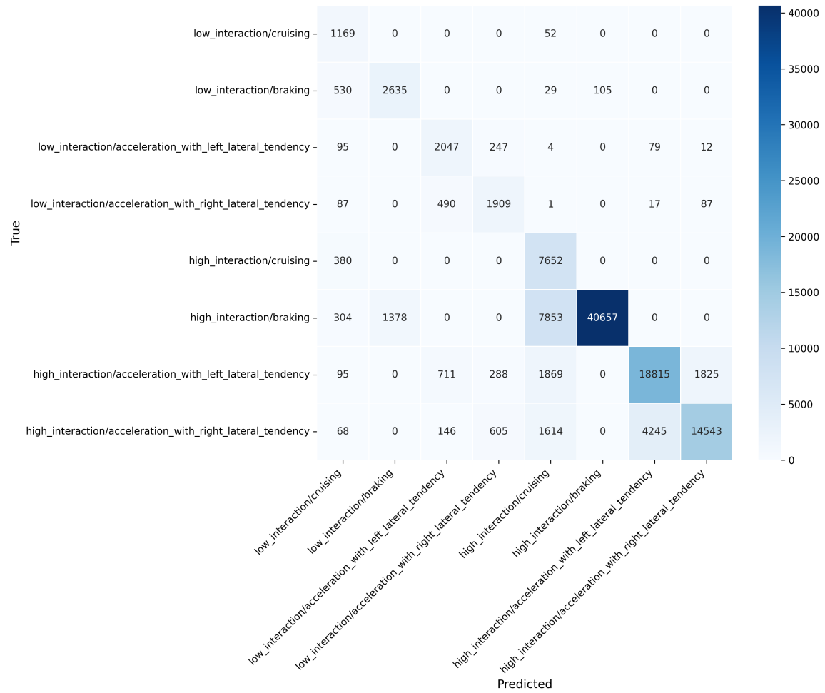
FIGURE 8: Confusion matrix.
