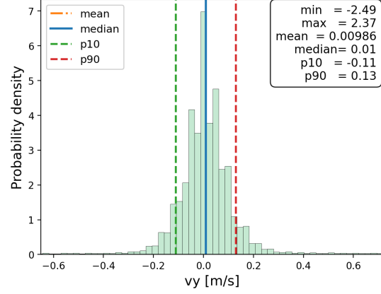
(f) Car: lateral velocity.
