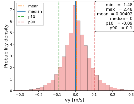
(h) Truck: lateral velocity.
