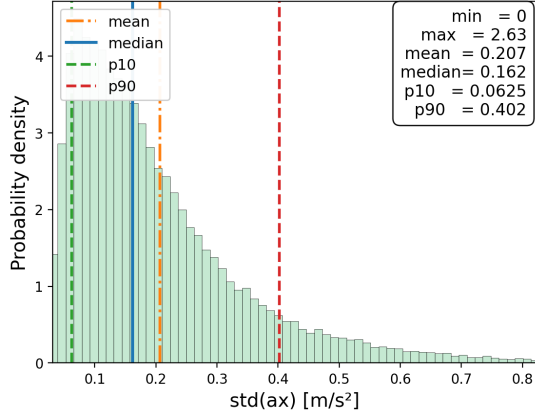
(a) Car: variability of longitudinal acceleration.
