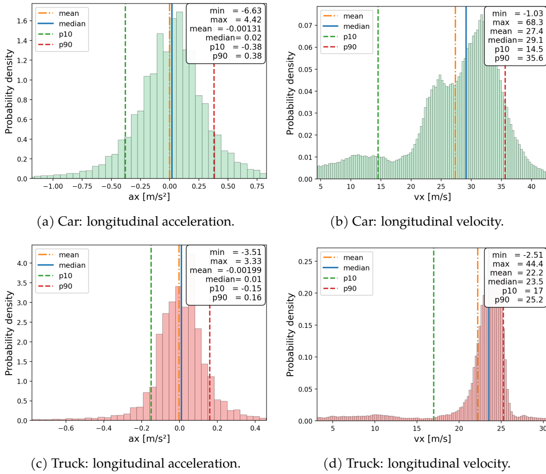
Figure A.1.: Class-wise frame-level distributions of the main kinematic variables.
