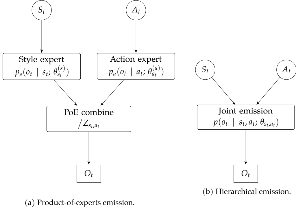
Figure 4.9.: Emission model variants considered in the proposed DBN.
