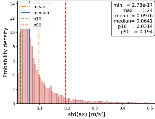
(c) Truck: variability of longitudinal acceleration.
