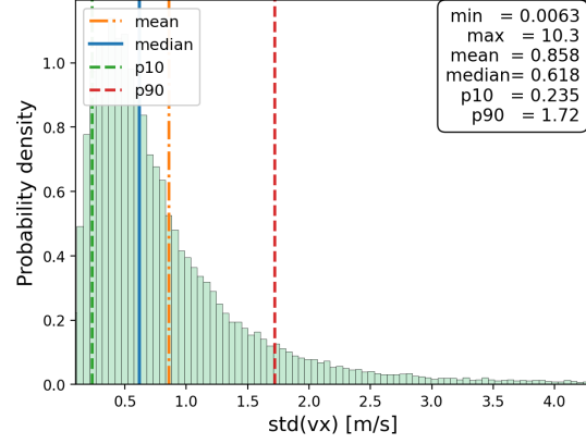
(b) Car: variability of longitudinal velocity.
