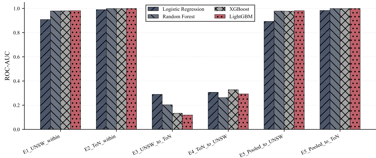
Baseline ROC-AUC by Protocol
