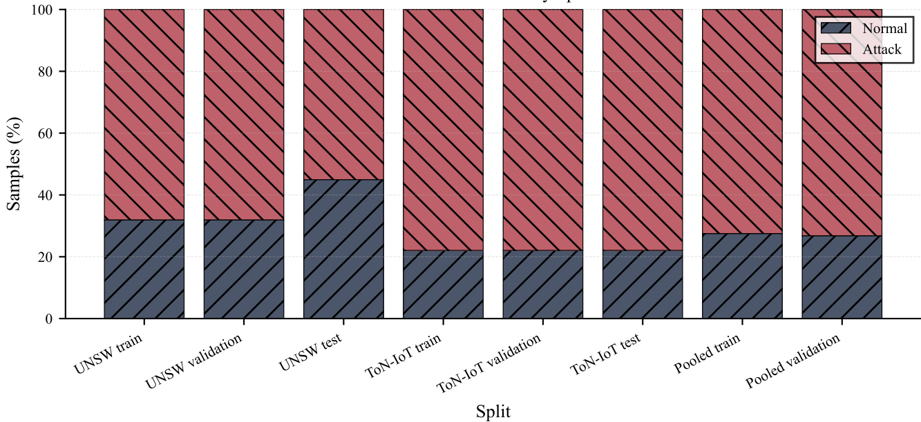
Class Distribution by Split
