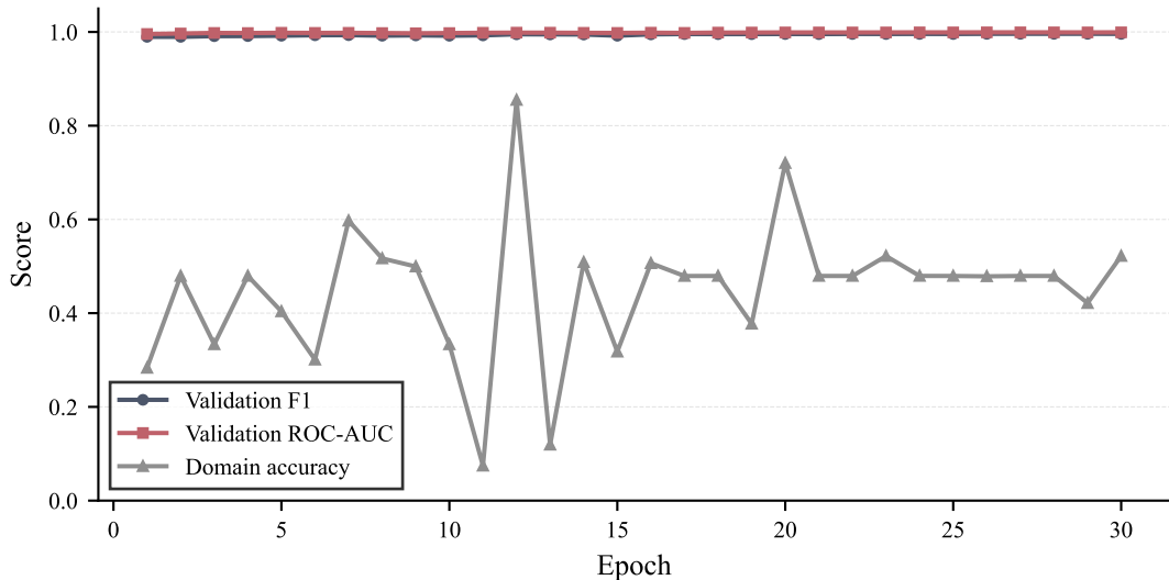
Training Curve: DANN_ToN_to_UNSW
