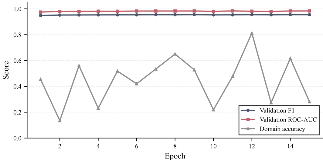
Training Curve: DANN_UNSW_to_ToN
