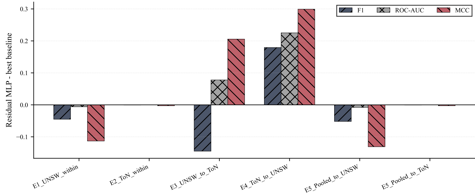
Residual MLP Metric Differences
