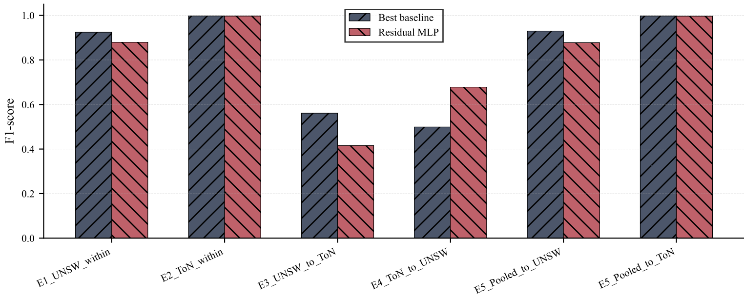
Residual MLP and Best Baseline
