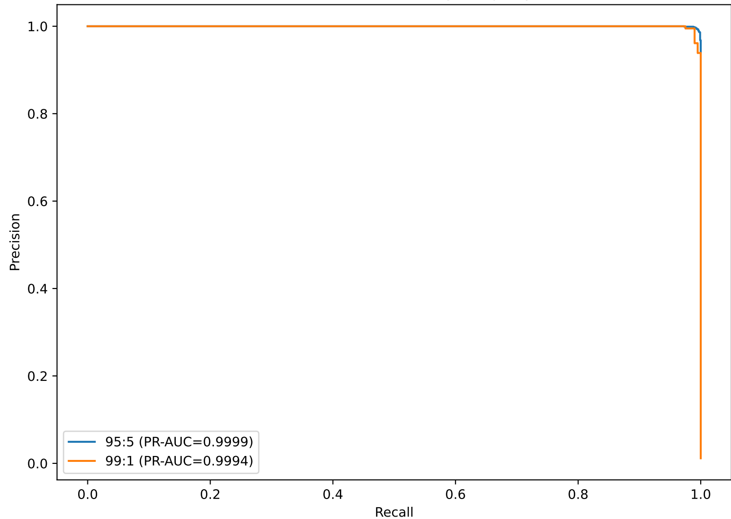
Precision-Recall curves under benign-majority scenarios
