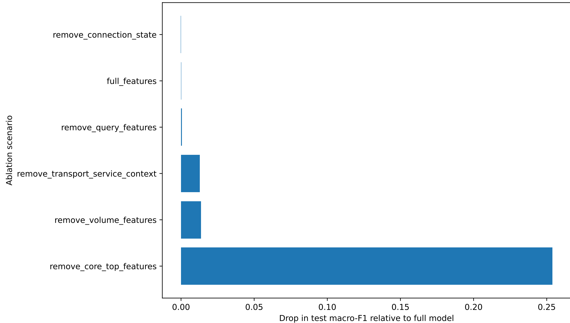
Macro-F1 drop under feature-group ablation
