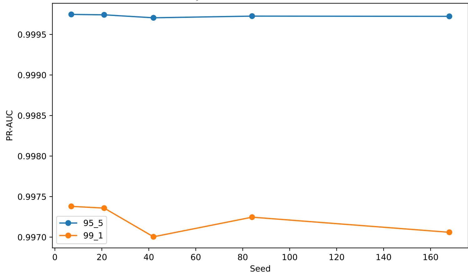
Binary PR-AUC across random seeds
