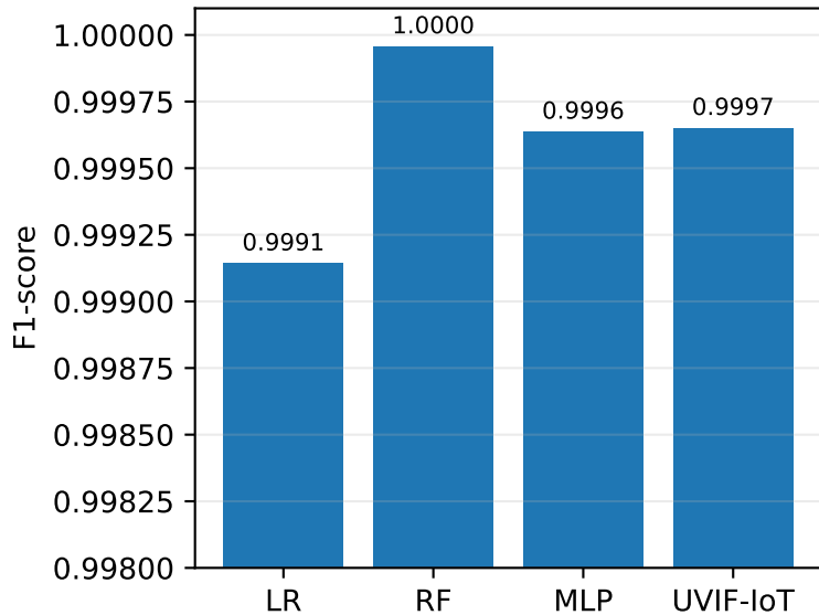
Detection
