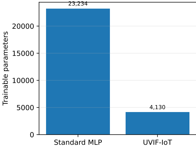
Model size
