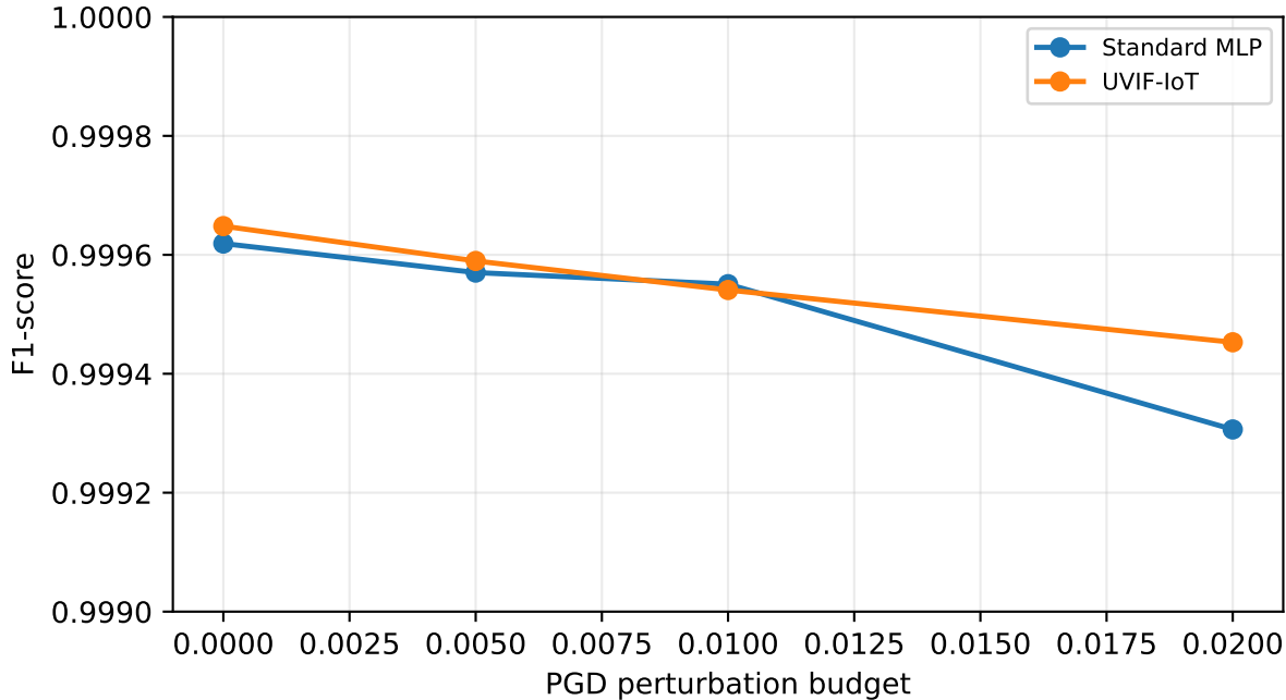
Robustness under PGD
