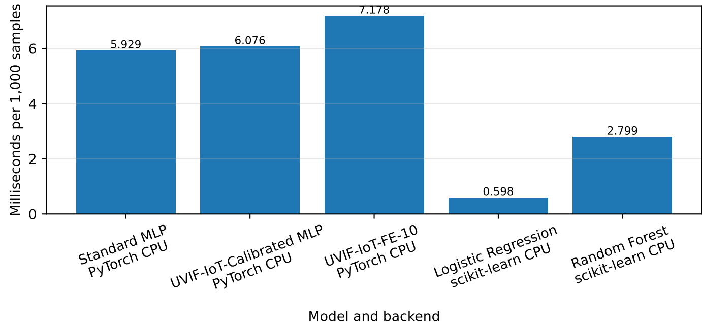
Measured Inference Time on Pilot Test Subset
