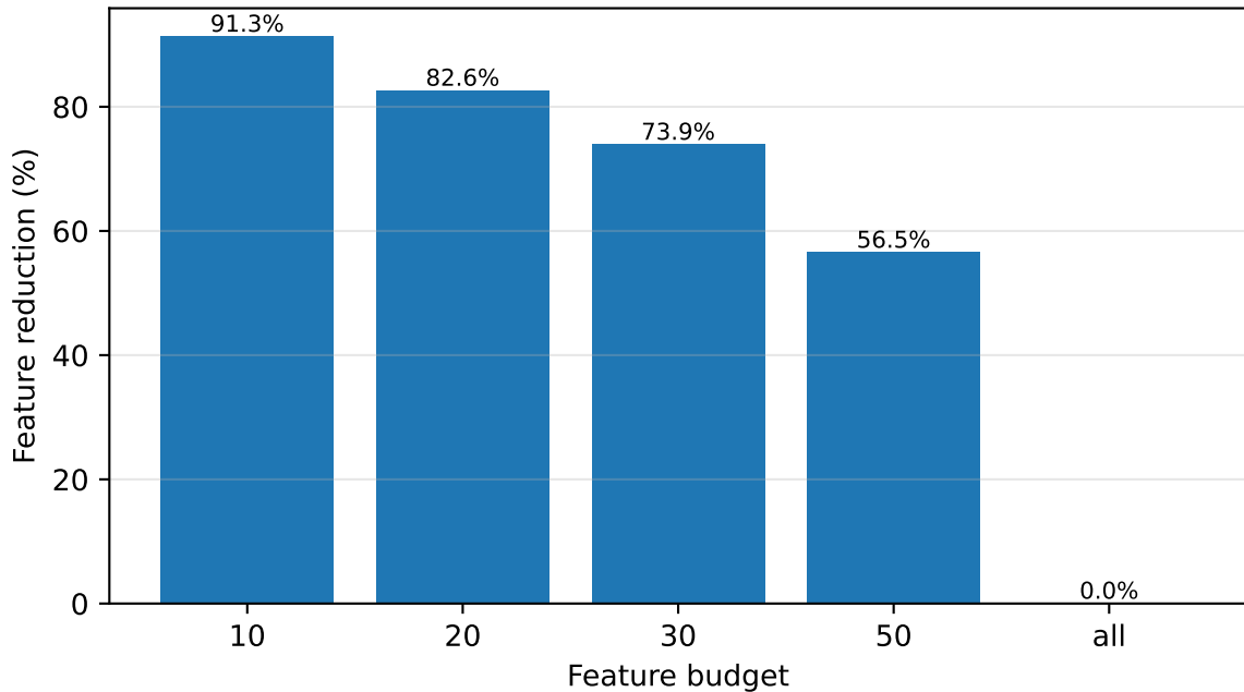
Feature Reduction by Budget
