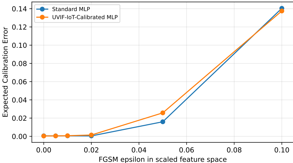
FGSM Robustness: ECE vs Perturbation Size
