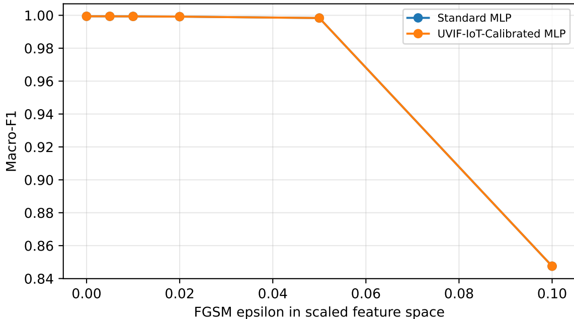
FGSM Robustness: Macro-F1 vs Perturbation Size
