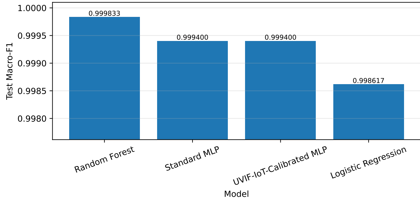
Clean Detection Performance
